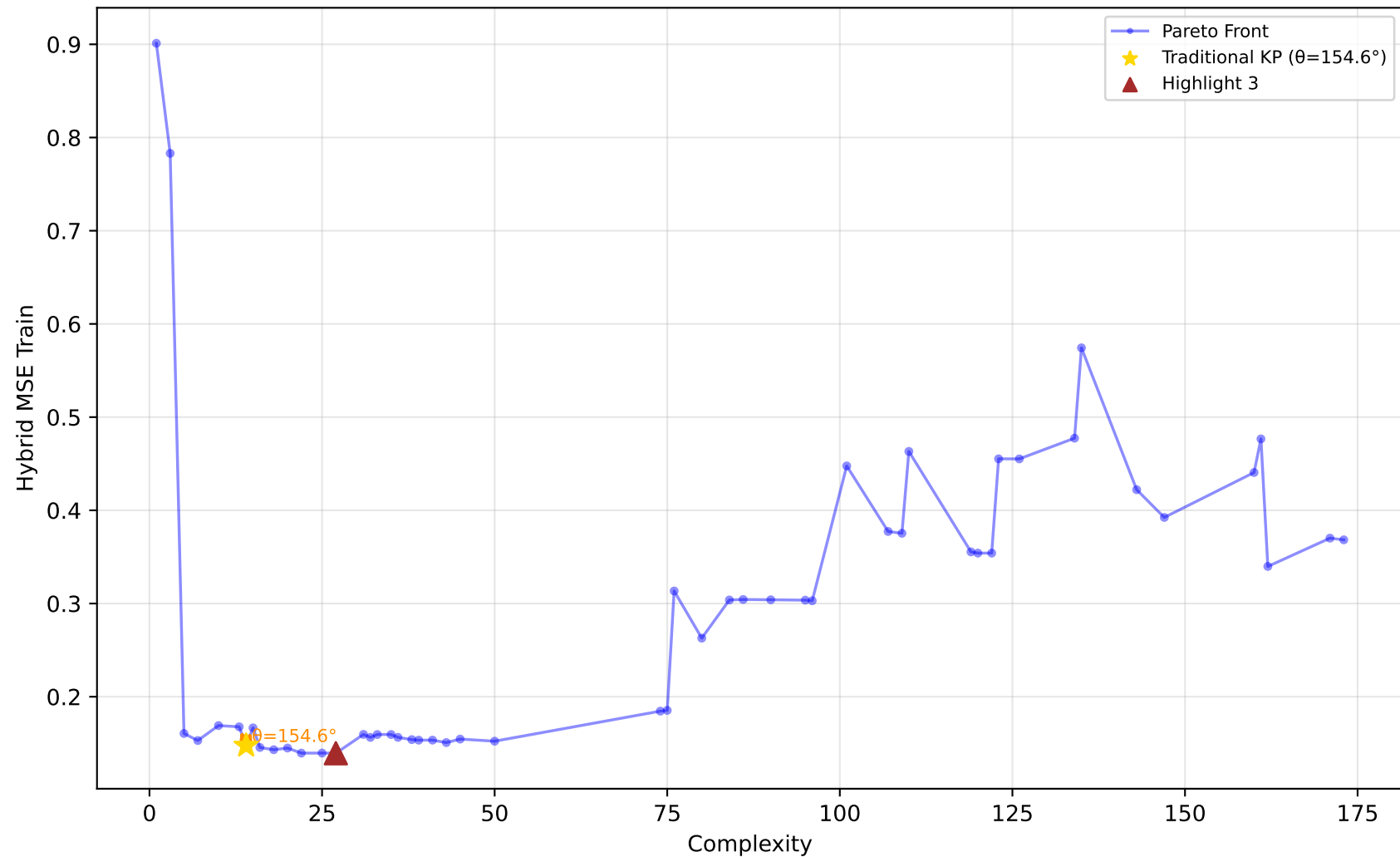
712_chscase_geyser1 - Run 1 - MVP - Hybrid MSE Train \lambda_1=0.20, \lambda_2=1.00, \lambda_3=1.00 | Difficulty: 1.00 | Method: hmr
