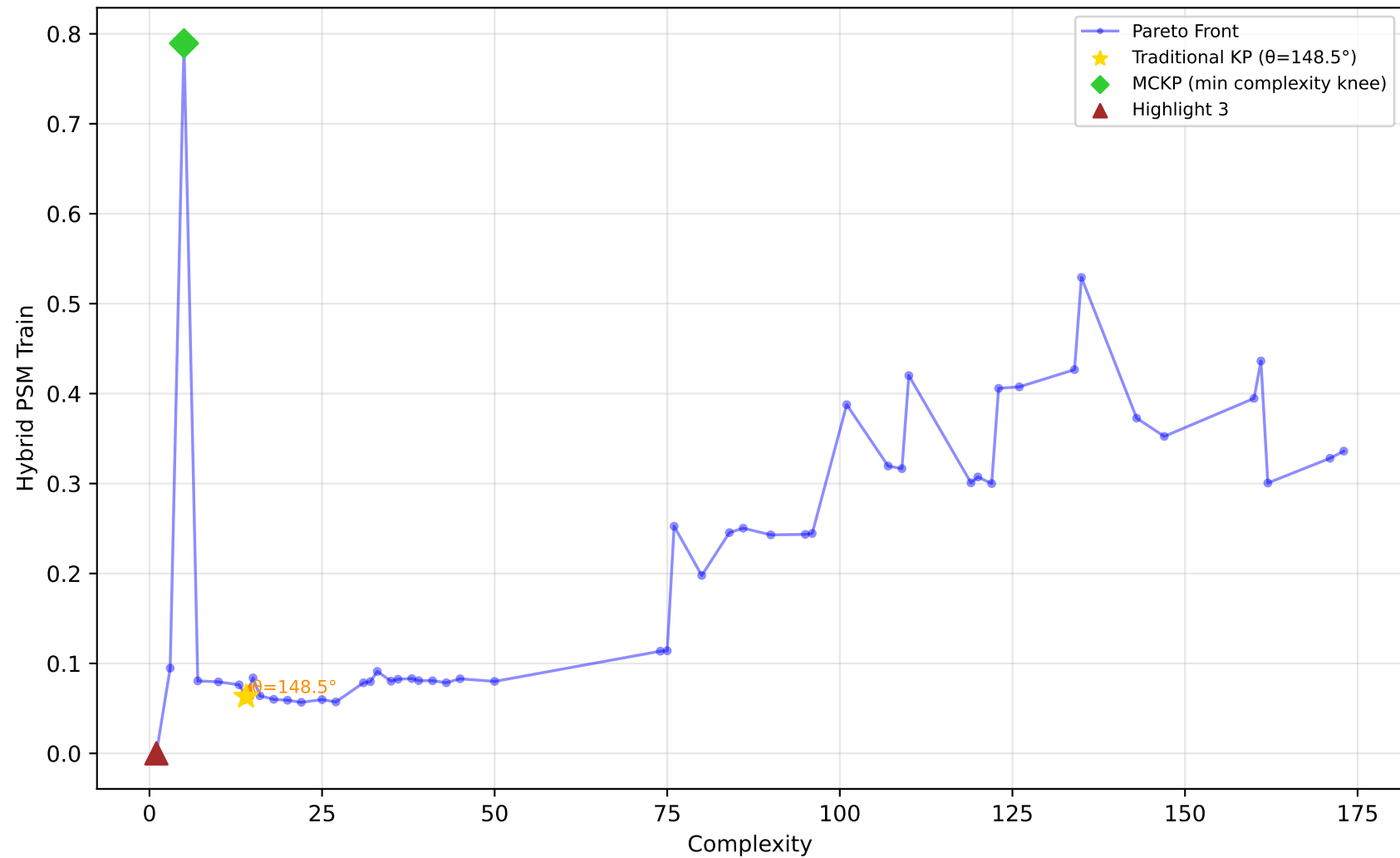
712_chscase_geyser1 - Run 1 - MVP - Hybrid PSM Train \lambda_1=0.20, \lambda_2=1.00, \lambda_3=1.00 | Difficulty: 1.00 | Method: hmr
