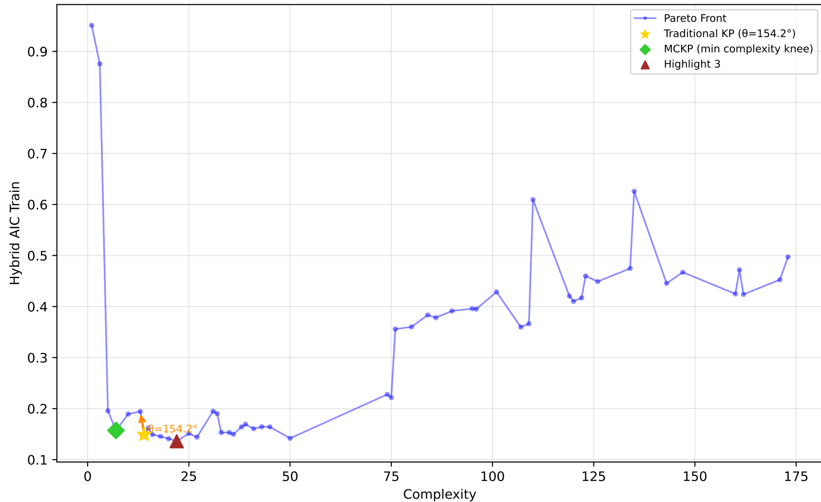
712_chscase_geyser1 - Run 1 - SVP - Hybrid AIC Train \lambda_1=0.00, \lambda_2=1.00, \lambda_3=1.00 | Difficulty: 1.00 | Method: hmr
