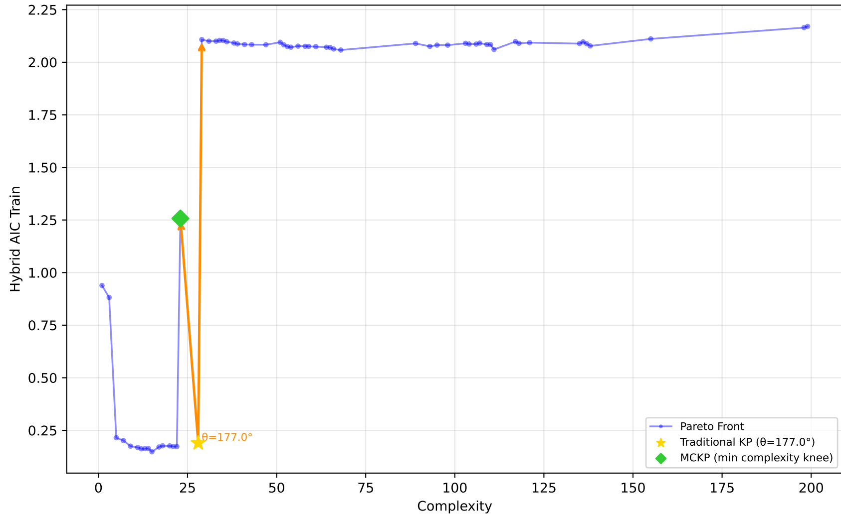
712_chscase_geyser1 - Run 20 - MVP - Hybrid AIC Train \lambda_1=0.20, \lambda_2=1.00, \lambda_3=1.00 | Difficulty: 1.00 | Method: hmr
