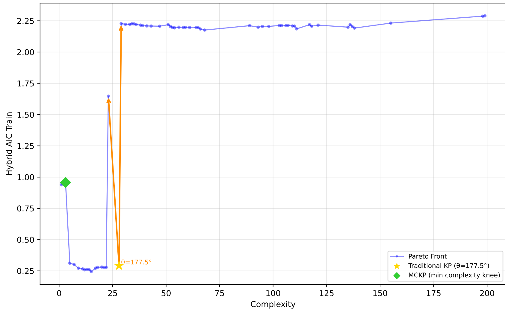
712_chscase_geyser1 - Run 20 - MVP - Hybrid AIC Train \lambda_1=1.00 , \lambda_2=1.00 , \lambda_3=1.00 | Difficulty: 1.00 | Method: hmr
