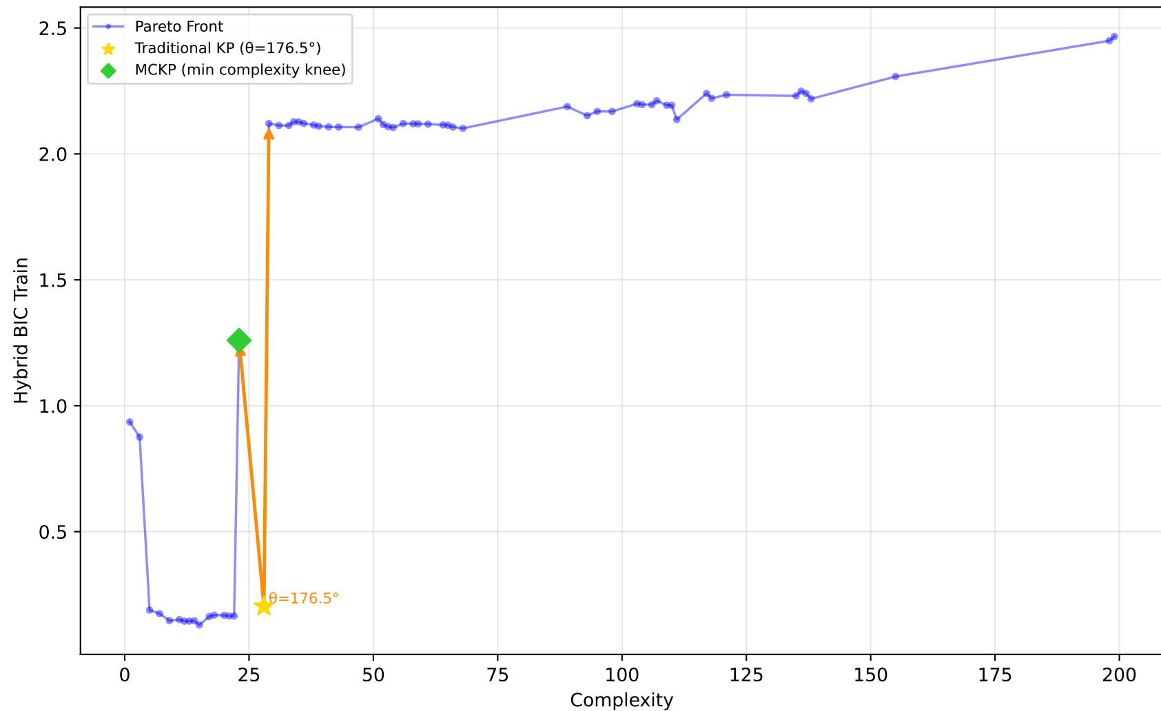
712_chscase_geyser1 - Run 20 - MVP - Hybrid BIC Train \lambda_1=0.20, \lambda_2=1.00, \lambda_3=1.00 | Difficulty: 1.00 | Method: hmr
