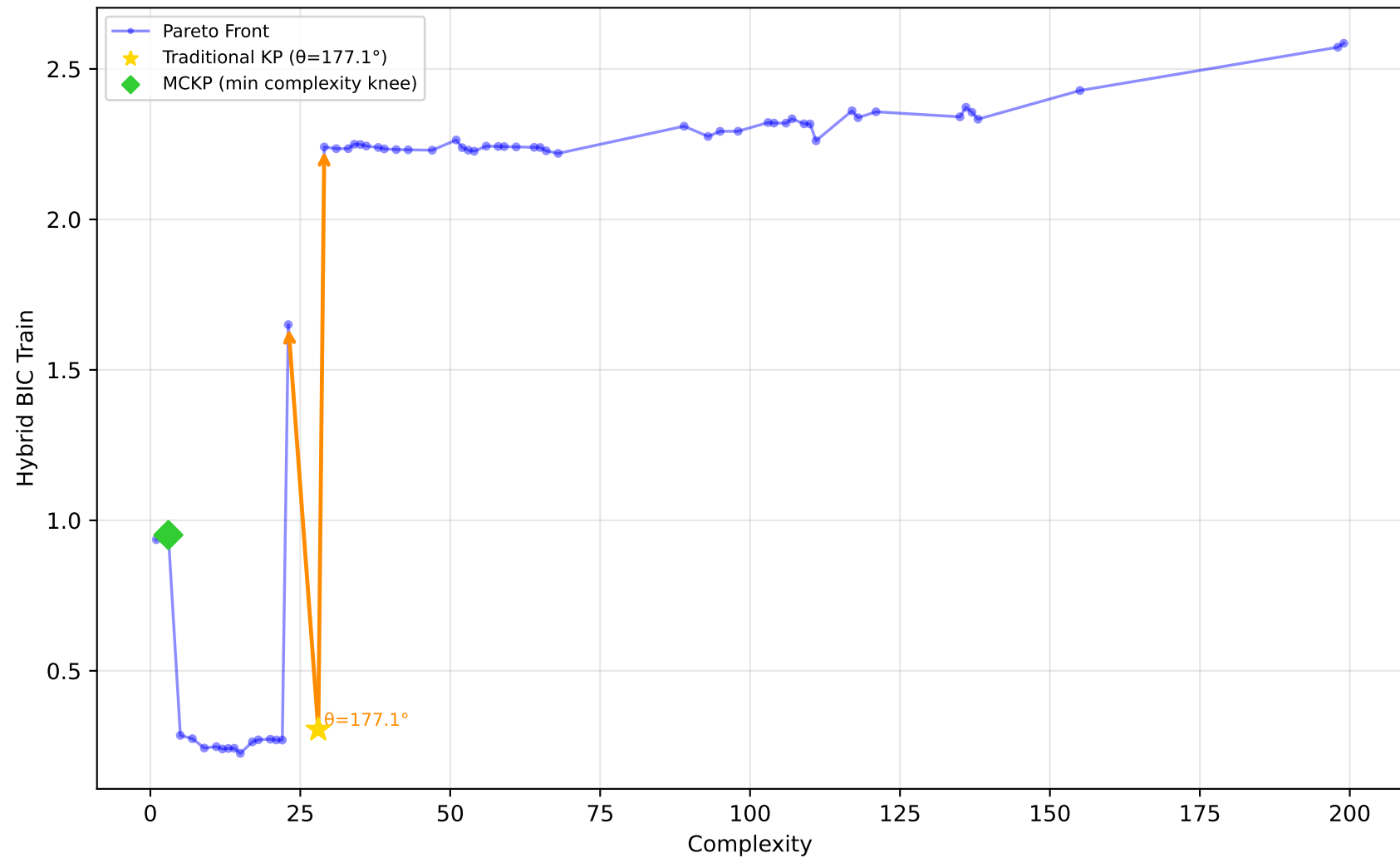
712_chscase_geyser1 - Run 20 - MVP - Hybrid BIC Train \lambda_1=1.00, \lambda_2=1.00, \lambda_3=1.00 | Difficulty: 1.00 | Method: hmr
