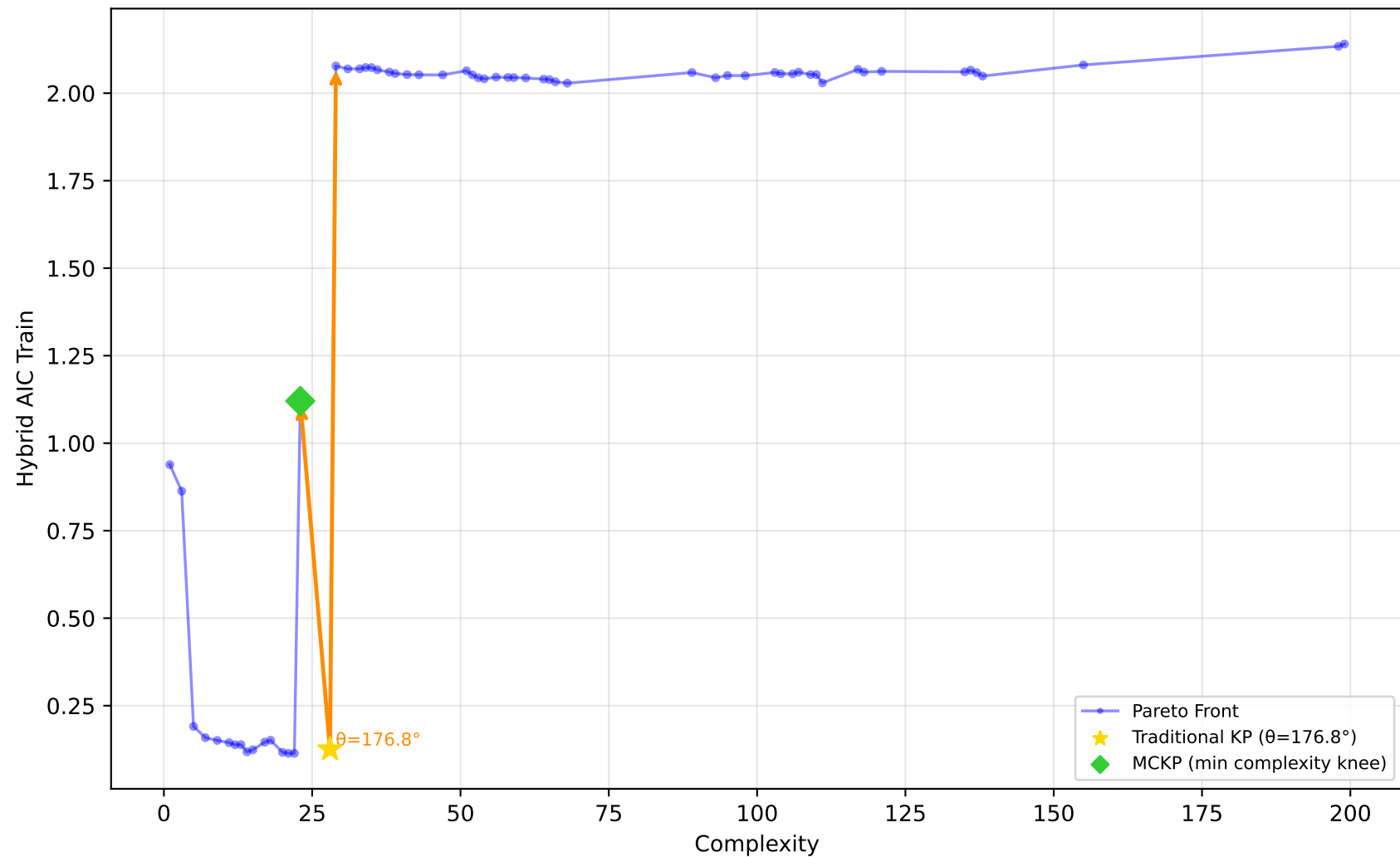
712_chscase_geyser1 - Run 20 - SVP - Hybrid AIC Train \lambda_1=0.00, \lambda_2=1.00, \lambda_3=1.00 | Difficulty: 1.00 | Method: hmr
