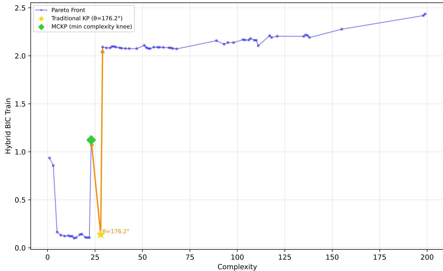
712_chscase_geyser1 - Run 20 - SVP - Hybrid BIC Train \lambda_1=0.00, \lambda_2=1.00, \lambda_3=1.00 | Difficulty: 1.00 | Method: hmr
