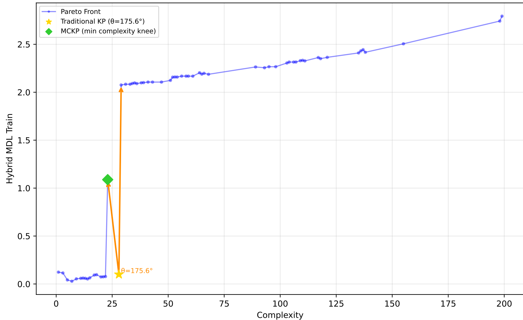
712_chscase_geyser1 - Run 20 - SVP - Hybrid MDL Train \lambda_1=0.00, \lambda_2=1.00, \lambda_3=1.00 | Difficulty: 1.00 | Method: hmr
