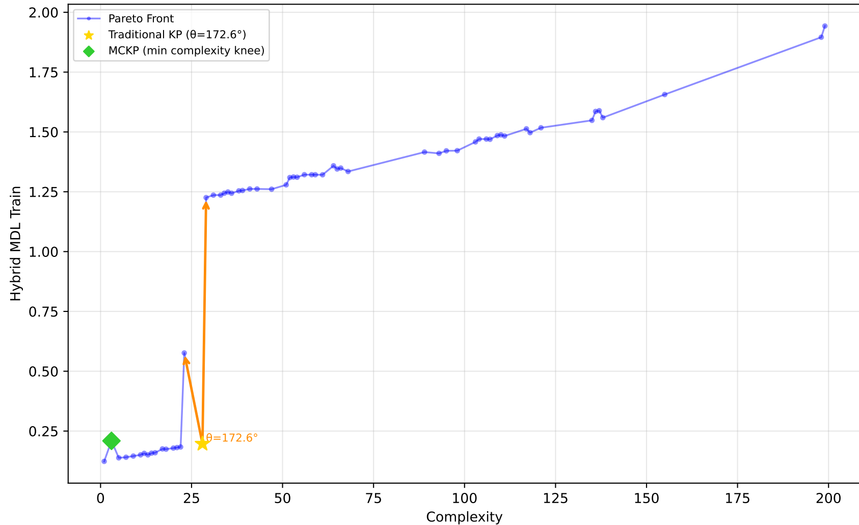
712_chscase_geyser1 - Run 20 - SVP - Hybrid MDL Train \lambda_1=1.00, \lambda_2=1.00, \lambda_3=0.00 | Difficulty: 1.00 | Method: hmr
