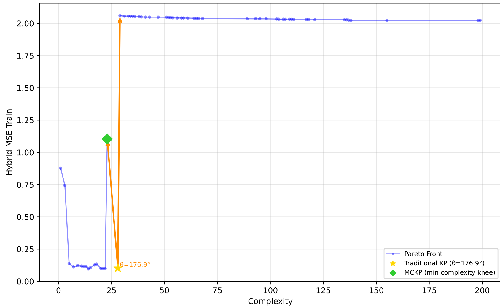
712_chscase_geyser1 - Run 20 - SVP - Hybrid MSE Train \lambda_1=0.00, \lambda_2=1.00, \lambda_3=1.00 | Difficulty: 1.00 | Method: hmr
