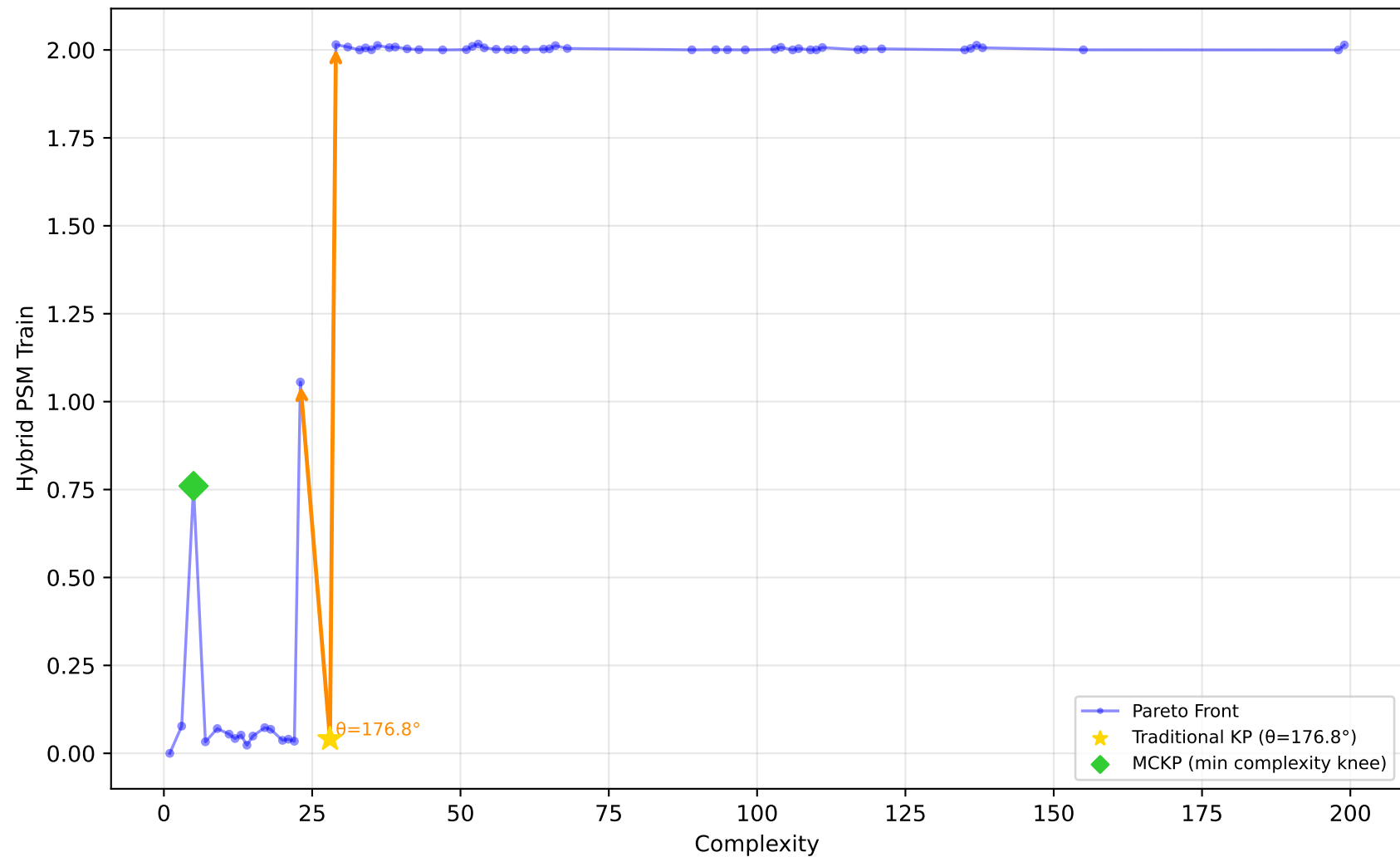
712_chscase_geyser1 - Run 20 - SVP - Hybrid PSM Train \lambda_1=0.00, \lambda_2=1.00, \lambda_3=1.00 | Difficulty: 1.00 | Method: hmr
