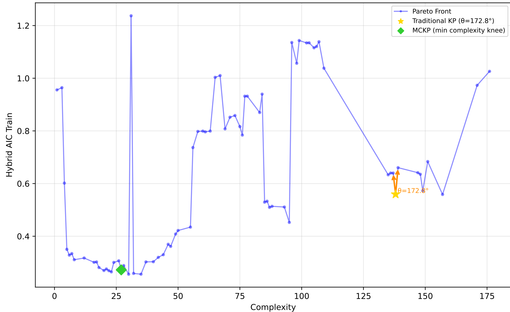
712_chscase_geyser1 - Run 21 - MVP - Hybrid AIC Train \lambda_1=1.00, \lambda_2=1.00, \lambda_3=1.00 | Difficulty: 0.48 | Method: mckp
