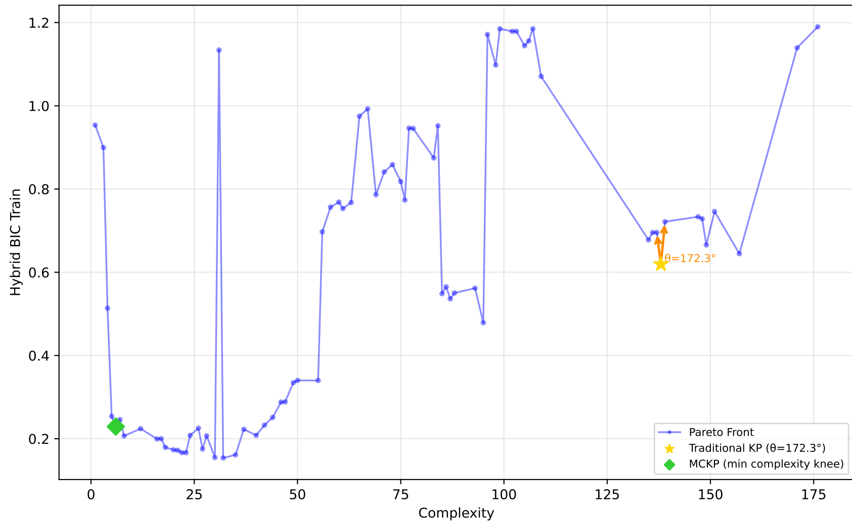
712_chscase_geyser1 - Run 21 - MVP - Hybrid BIC Train \lambda_1=0.20 , \lambda_2=1.00 , \lambda_3=1.00 | Difficulty: 0.48 | Method: mckp
