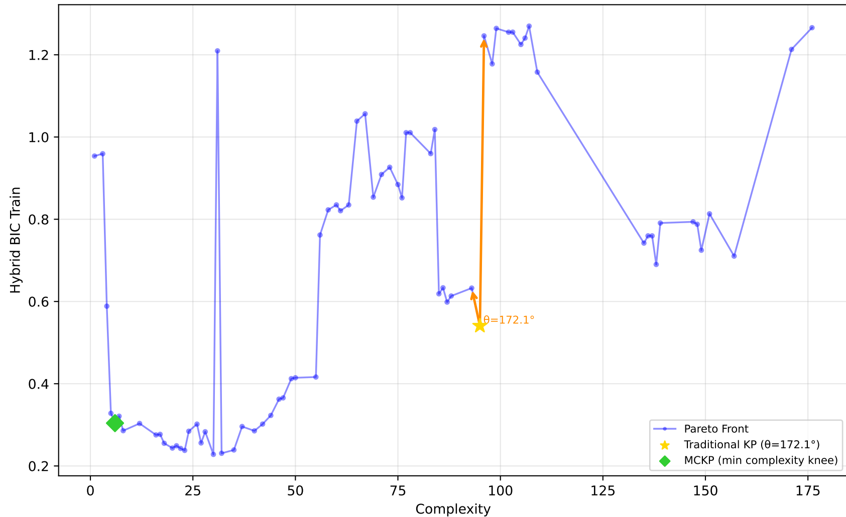
712_chscase_geyser1 - Run 21 - MVP - Hybrid BIC Train \lambda_1=1.00, \lambda_2=1.00, \lambda_3=1.00 | Difficulty: 0.48 | Method: mckp
