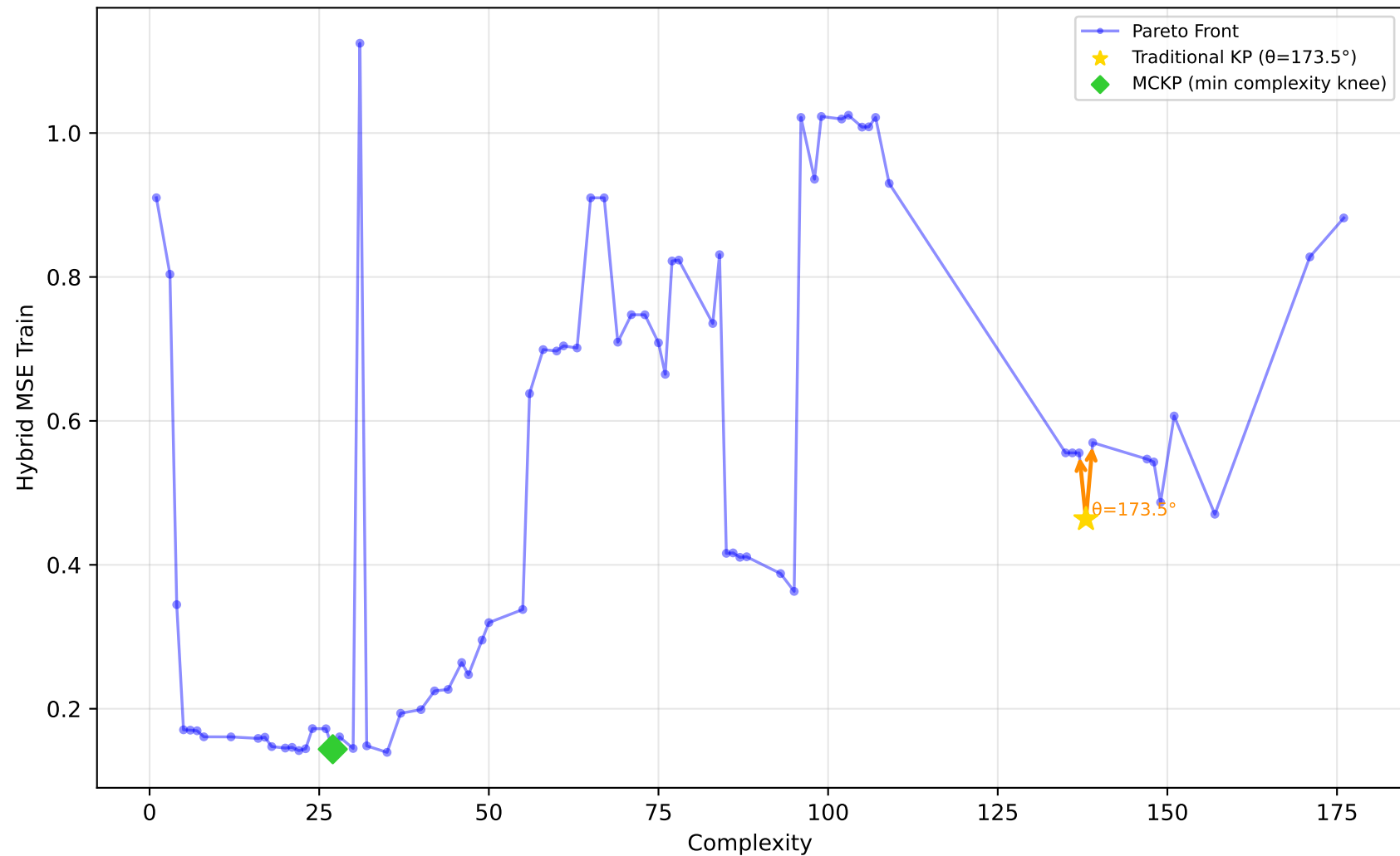
712_chscase_geyser1 - Run 21 - MVP - Hybrid MSE Train \lambda_1=0.20 , \lambda_2=1.00 , \lambda_3=1.00 | Difficulty: 0.48 | Method: mckp
