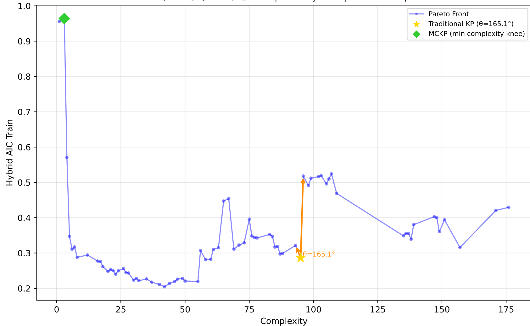
712_chscase_geyser1 - Run 21 - SVP - Hybrid AIC Train \lambda_1=1.00, \lambda_2=1.00, \lambda_3=0.00 | Difficulty: 0.48 | Method: mckp
