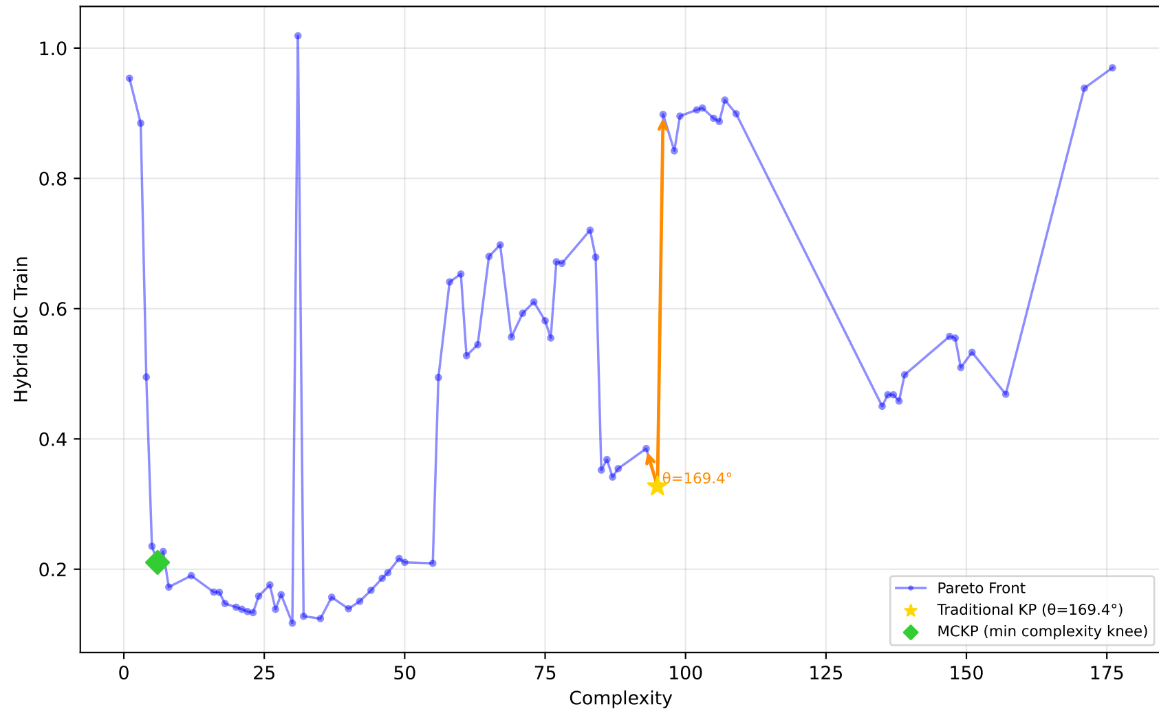
712_chscase_geyser1 - Run 21 - SVP - Hybrid BIC Train \lambda_1=0.00 , \lambda_2=1.00 , \lambda_3=1.00 | Difficulty: 0.48 | Method: mckp
