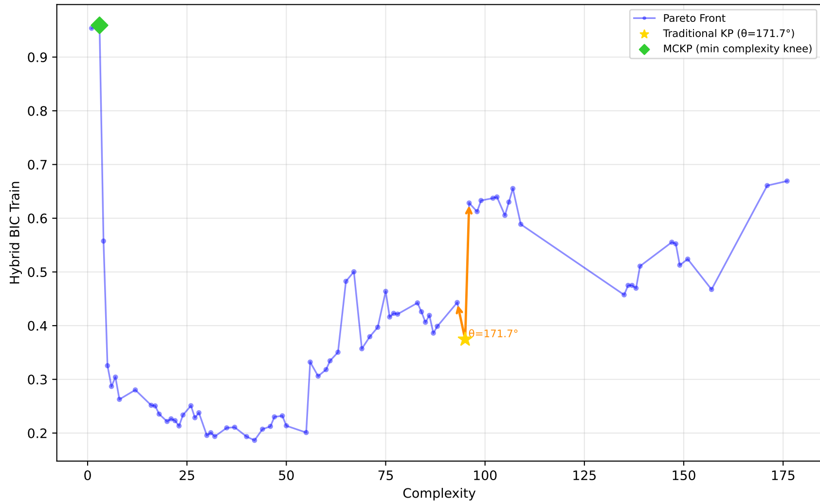
712_chscase_geyser1 - Run 21 - SVP - Hybrid BIC Train \lambda_1=1.00, \lambda_2=1.00, \lambda_3=0.00 | Difficulty: 0.48 | Method: mckp
