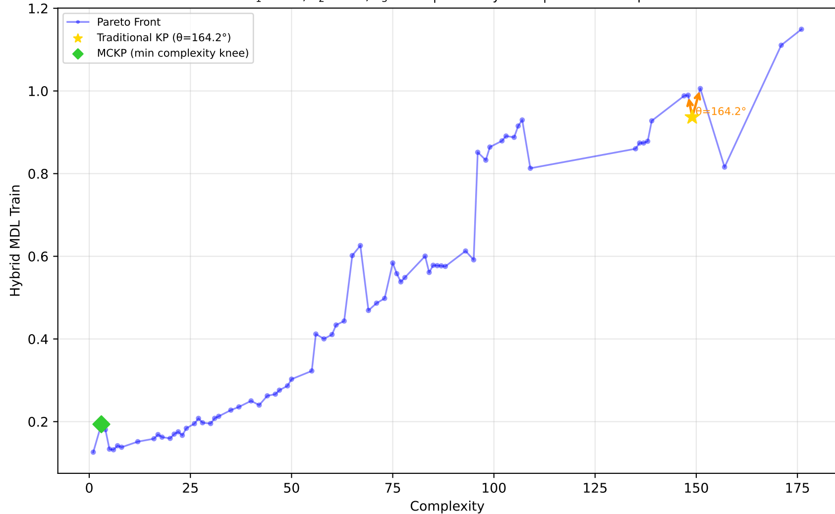
712_chscase_geyser1 - Run 21 - SVP - Hybrid MDL Train \lambda_1=1.00, \lambda_2=1.00, \lambda_3=0.00 | Difficulty: 0.48 | Method: mckp
