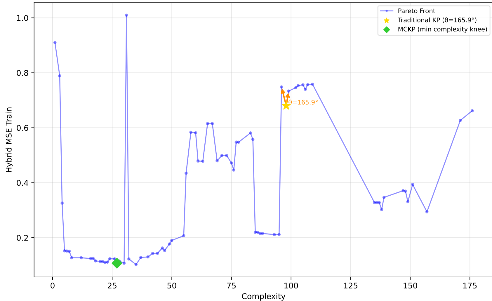
712_chscase_geyser1 - Run 21 - SVP - Hybrid MSE Train \lambda_1=0.00, \lambda_2=1.00, \lambda_3=1.00 | Difficulty: 0.48 | Method: mckp
