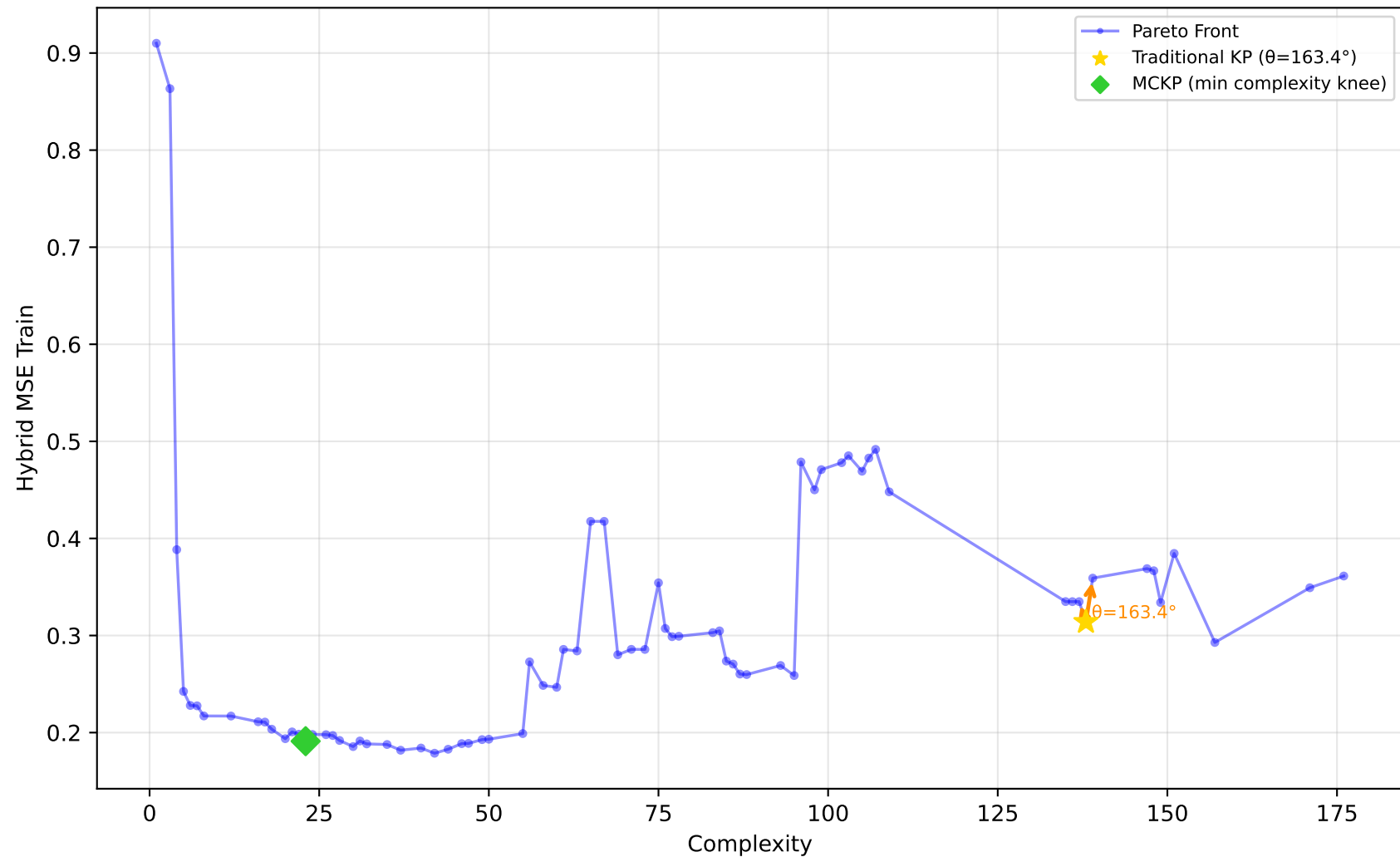
712_chscase_geyser1 - Run 21 - SVP - Hybrid MSE Train \lambda_1=1.00, \lambda_2=1.00, \lambda_3=0.00 | Difficulty: 0.48 | Method: mckp
