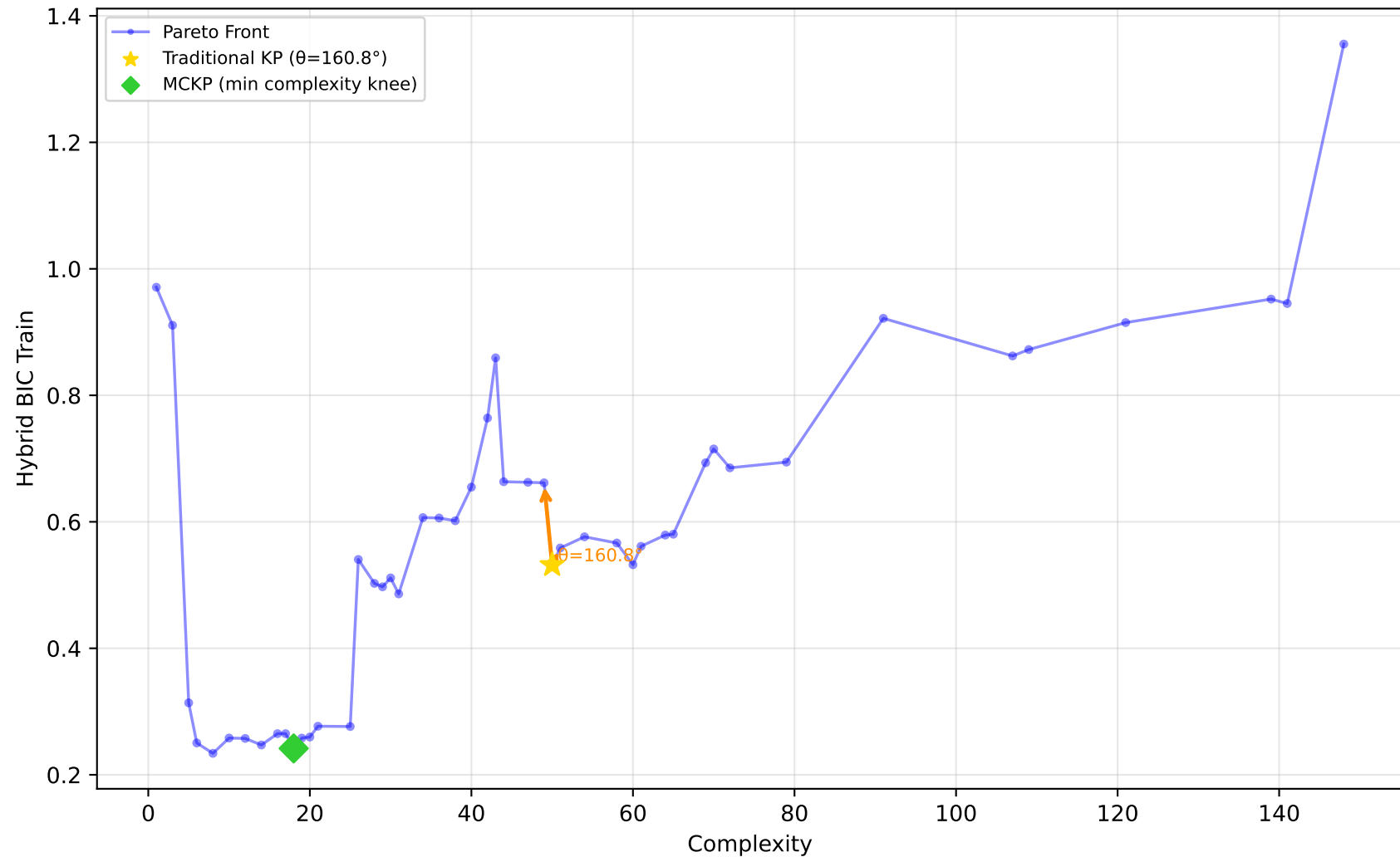
712_chscase_geyser1 - Run 22 - MVP - Hybrid BIC Train \lambda_1=0.20, \lambda_2=1.00, \lambda_3=1.00 | Difficulty: 0.62 | Method: hmr
