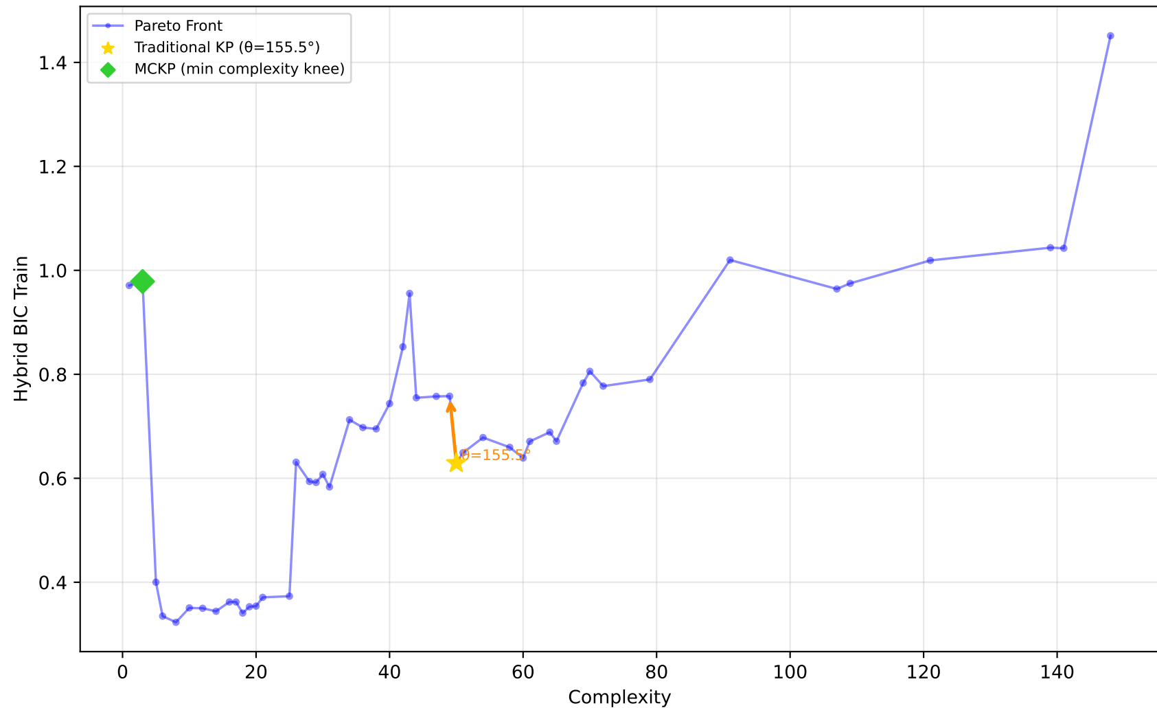
712_chscase_geyser1 - Run 22 - MVP - Hybrid BIC Train \lambda_1=1.00, \lambda_2=1.00, \lambda_3=1.00 | Difficulty: 0.62 | Method: hmr
