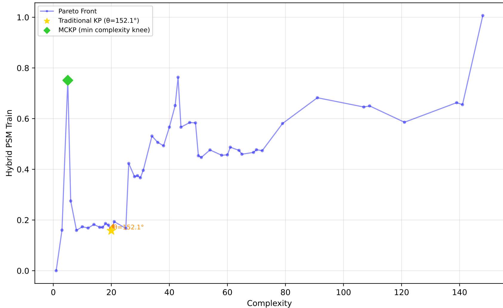
712_chscase_geyser1 - Run 22 - MVP - Hybrid PSM Train \lambda_1=1.00, \lambda_2=1.00, \lambda_3=1.00 | Difficulty: 0.62 | Method: hmr
