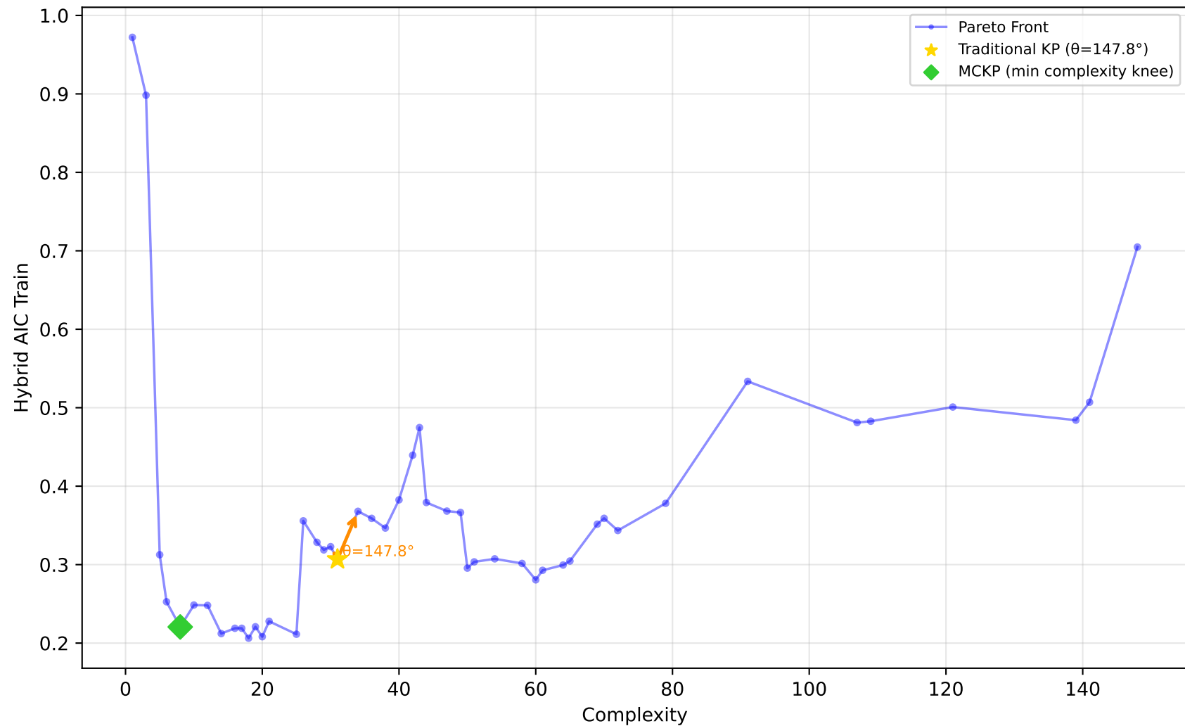
712_chscase_geyser1 - Run 22 - SVP - Hybrid AIC Train \lambda_1=0.00 , \lambda_2=1.00 , \lambda_3=1.00 | Difficulty: 0.62 | Method: hmr
