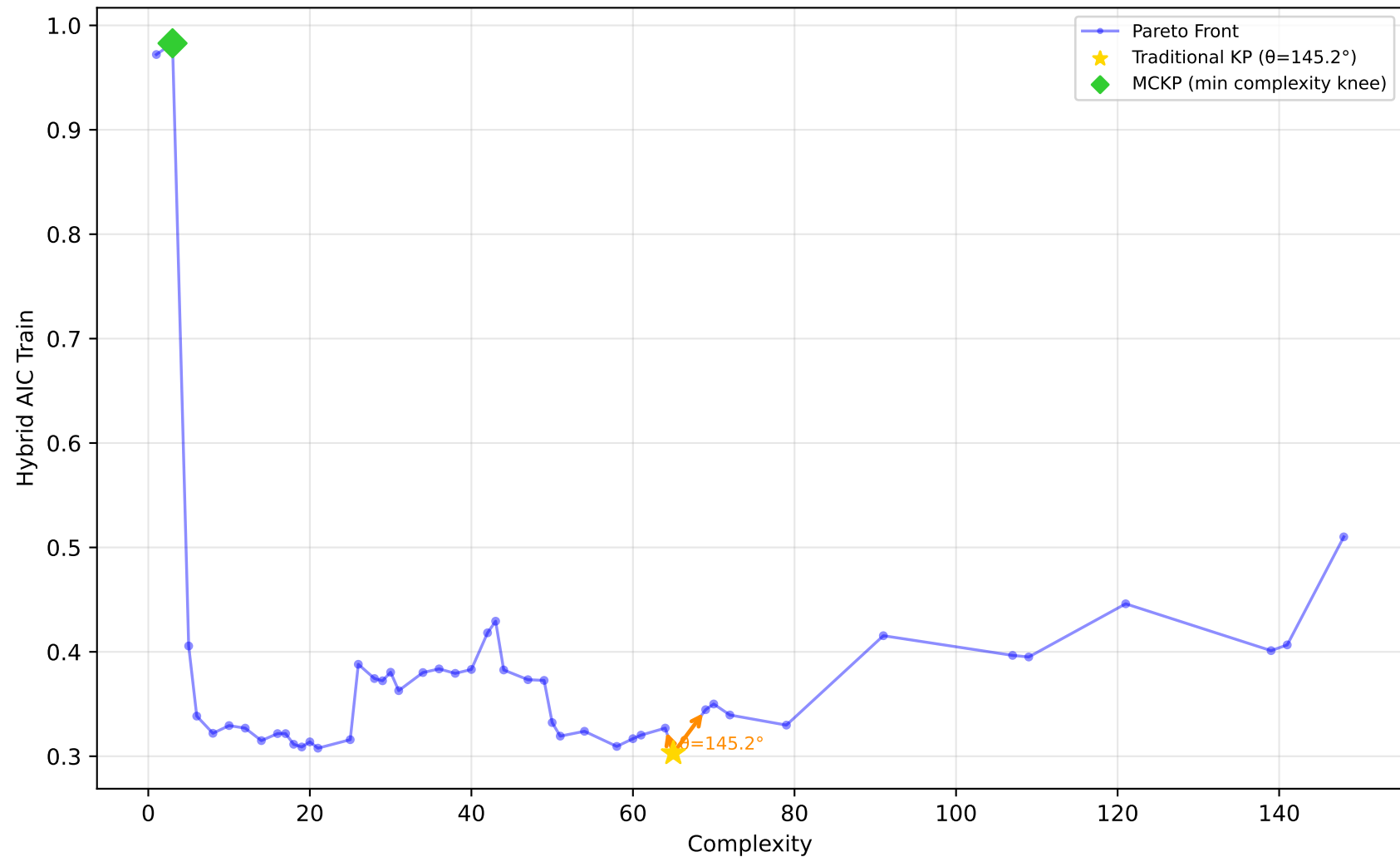
712_chscase_geyser1 - Run 22 - SVP - Hybrid AIC Train \lambda_1=1.00, \lambda_2=1.00, \lambda_3=0.00 | Difficulty: 0.62 | Method: hmr
