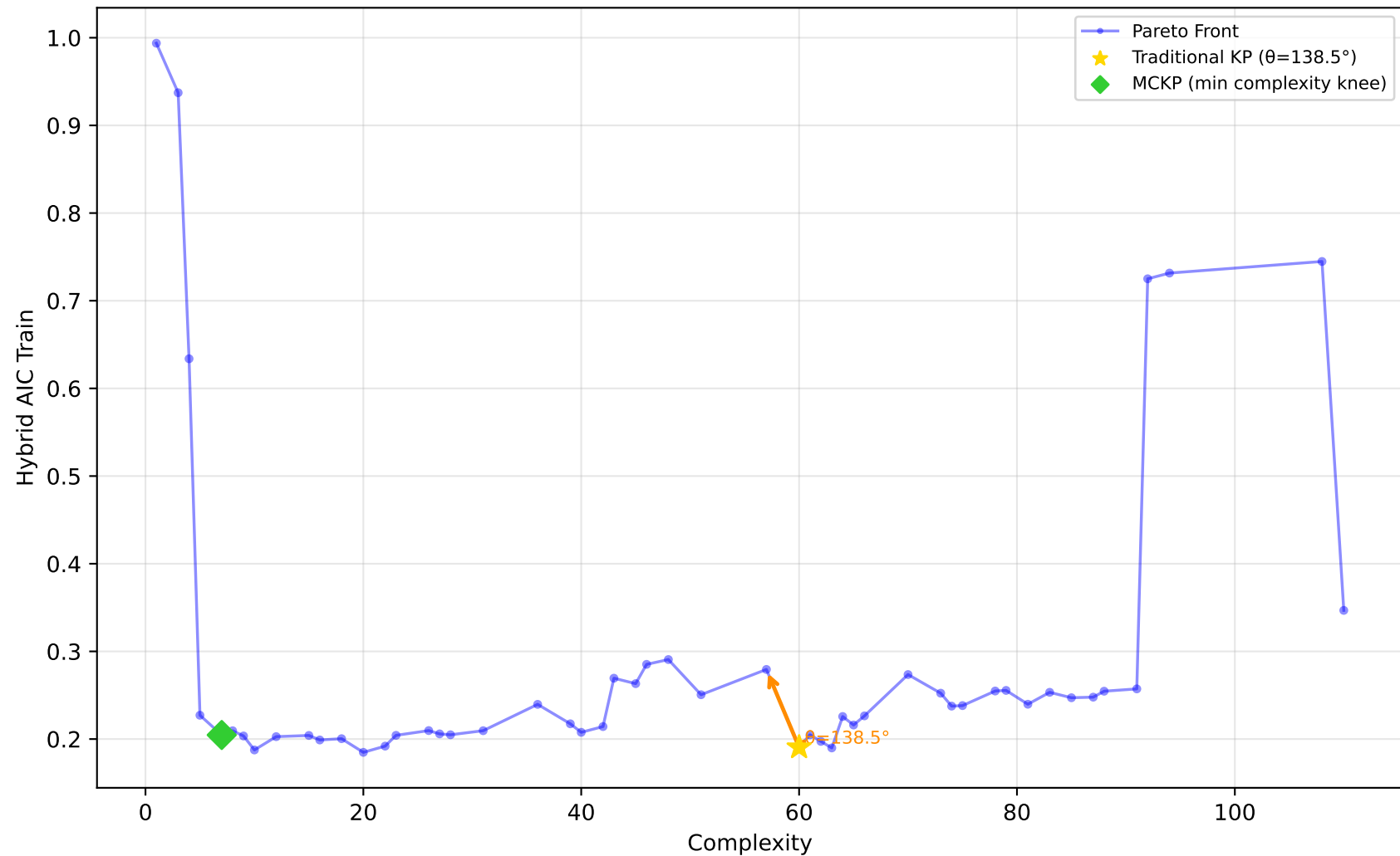
712_chscase_geyser1 - Run 23 - MVP - Hybrid AIC Train \lambda_1=0.20, \lambda_2=1.00, \lambda_3=1.00 | Difficulty: 0.63 | Method: hmr
