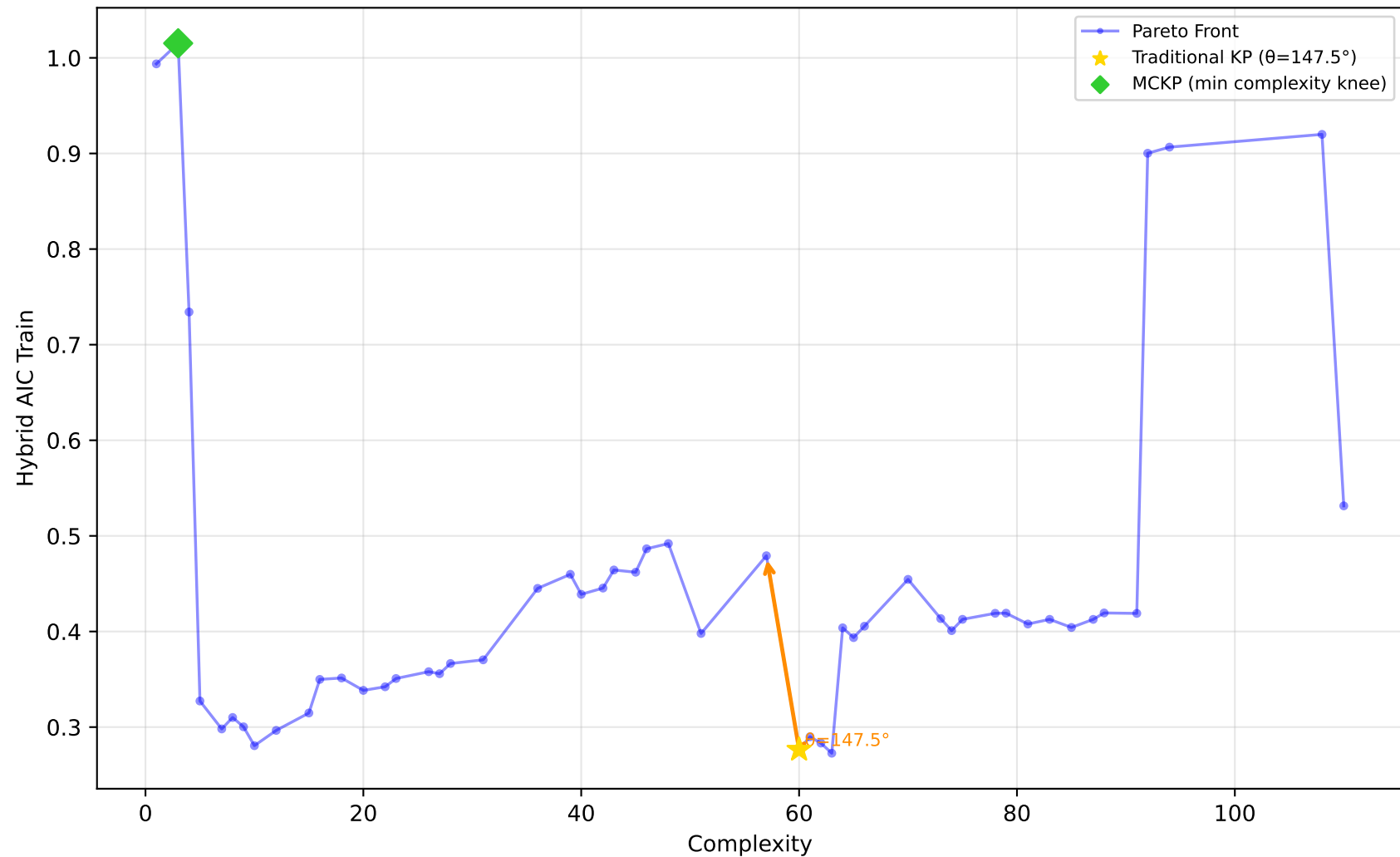
712_chscase_geyser1 - Run 23 - MVP - Hybrid AIC Train \lambda_1=1.00, \lambda_2=1.00, \lambda_3=1.00 | Difficulty: 0.63 | Method: hmr
