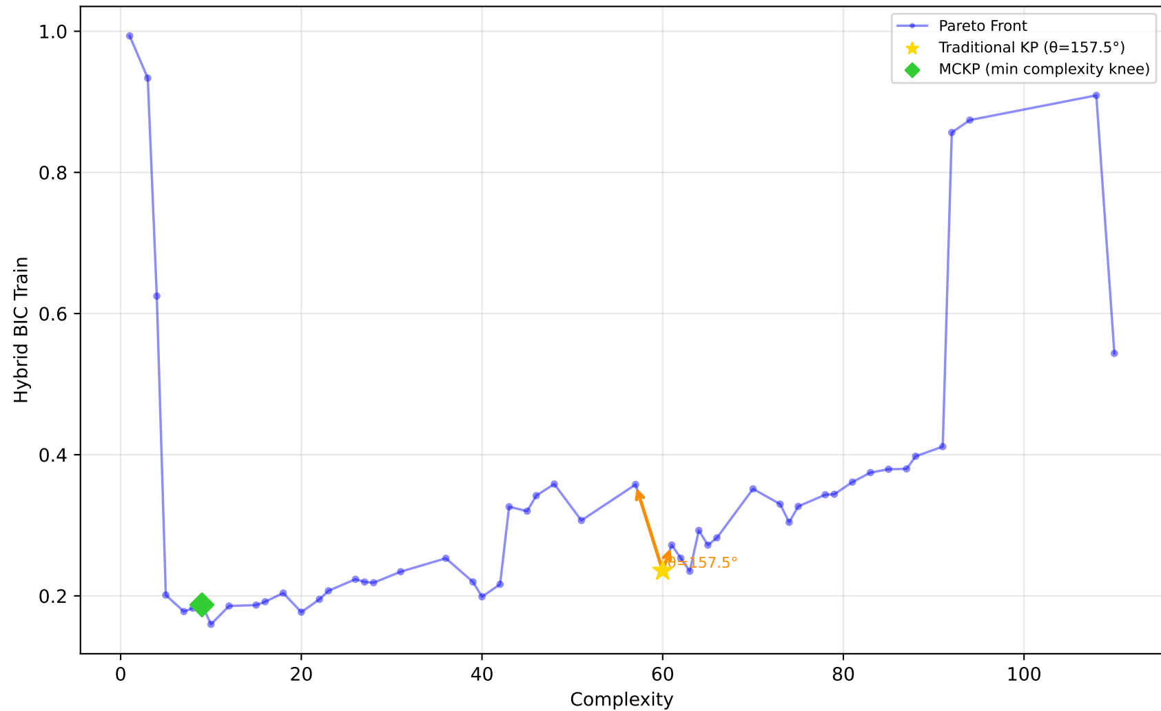
712_chscase_geyser1 - Run 23 - MVP - Hybrid BIC Train \lambda_1=0.20, \lambda_2=1.00, \lambda_3=1.00 | Difficulty: 0.63 | Method: hmr
