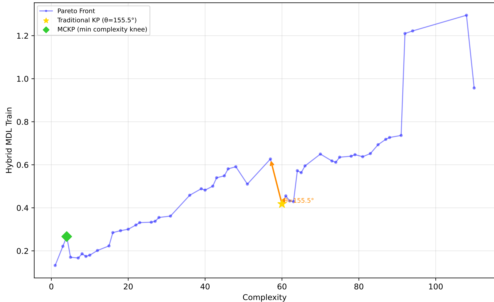
712_chscase_geyser1 - Run 23 - MVP - Hybrid MDL Train \lambda_1=1.00, \lambda_2=1.00, \lambda_3=1.00 | Difficulty: 0.63 | Method: hmr
