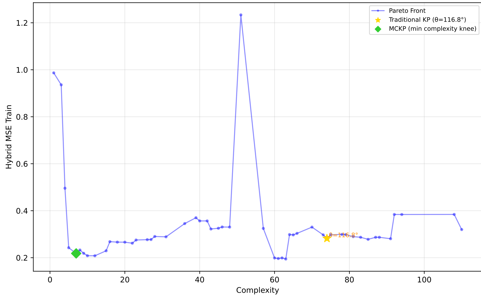
712_chscase_geyser1 - Run 23 - SVP - Hybrid MSE Train \lambda_1=1.00, \lambda_2=1.00, \lambda_3=0.00 | Difficulty: 0.63 | Method: hmr
