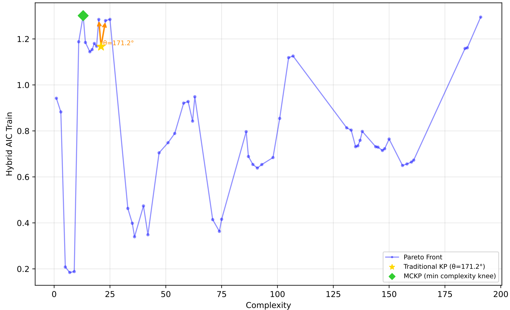
712_chscase_geyser1 - Run 24 - MVP - Hybrid AIC Train \lambda_1=0.20, \lambda_2=1.00, \lambda_3=1.00 | Difficulty: 0.35 | Method: mckp
