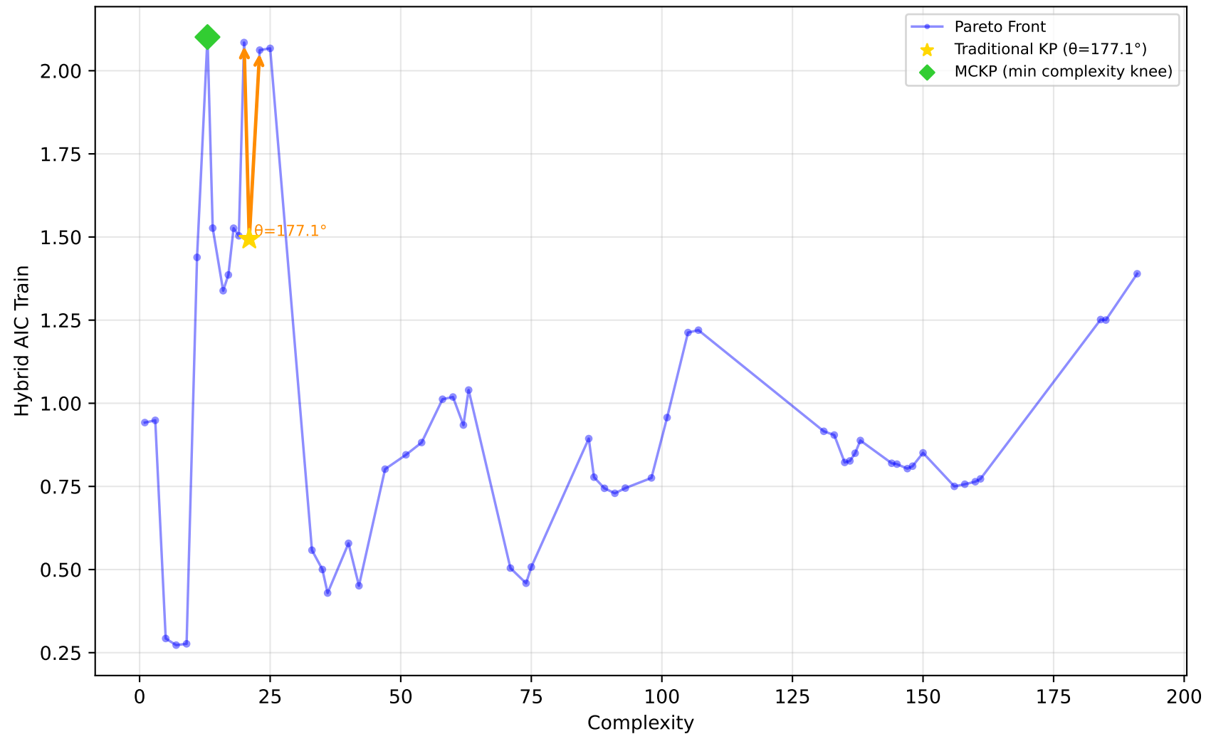
712_chscase_geyser1 - Run 24 - MVP - Hybrid AIC Train \lambda_1=1.00, \lambda_2=1.00, \lambda_3=1.00 | Difficulty: 0.35 | Method: mckp
