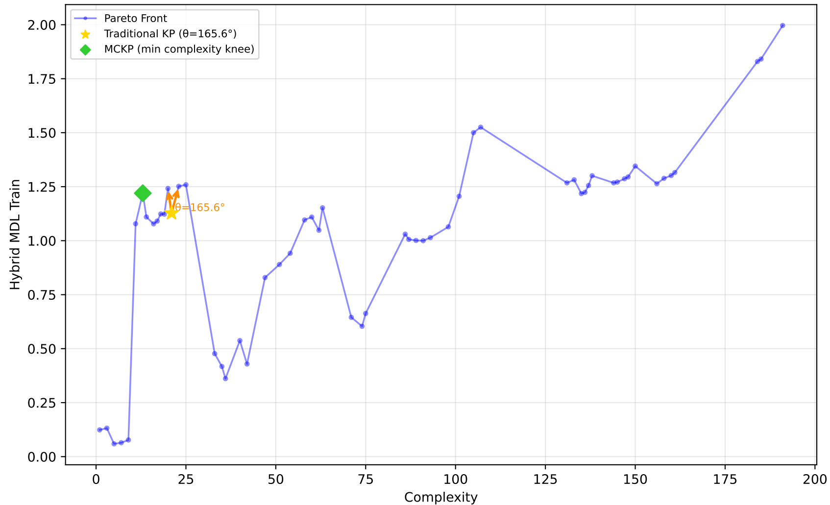
712_chscase_geyser1 - Run 24 - MVP - Hybrid MDL Train \lambda_1=0.20, \lambda_2=1.00, \lambda_3=1.00 | Difficulty: 0.35 | Method: mckp
