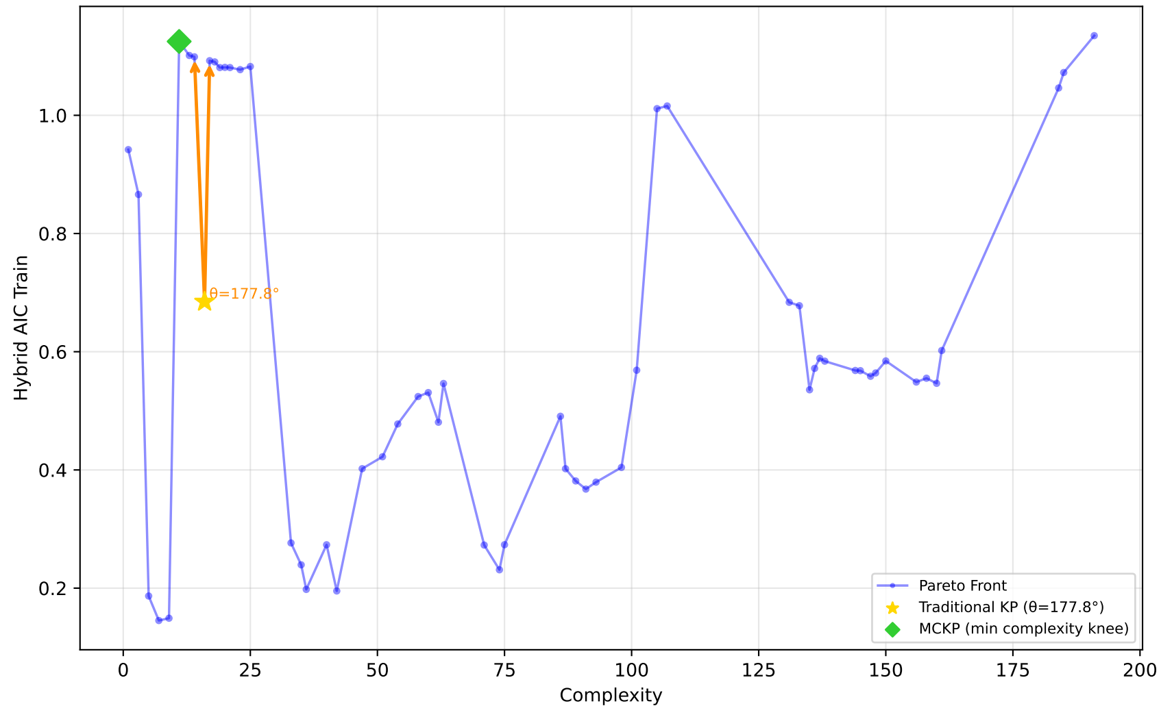
712_chscase_geyser1 - Run 24 - SVP - Hybrid AIC Train \lambda_1=0.00 , \lambda_2=1.00 , \lambda_3=1.00 | Difficulty: 0.35 | Method: mckp
