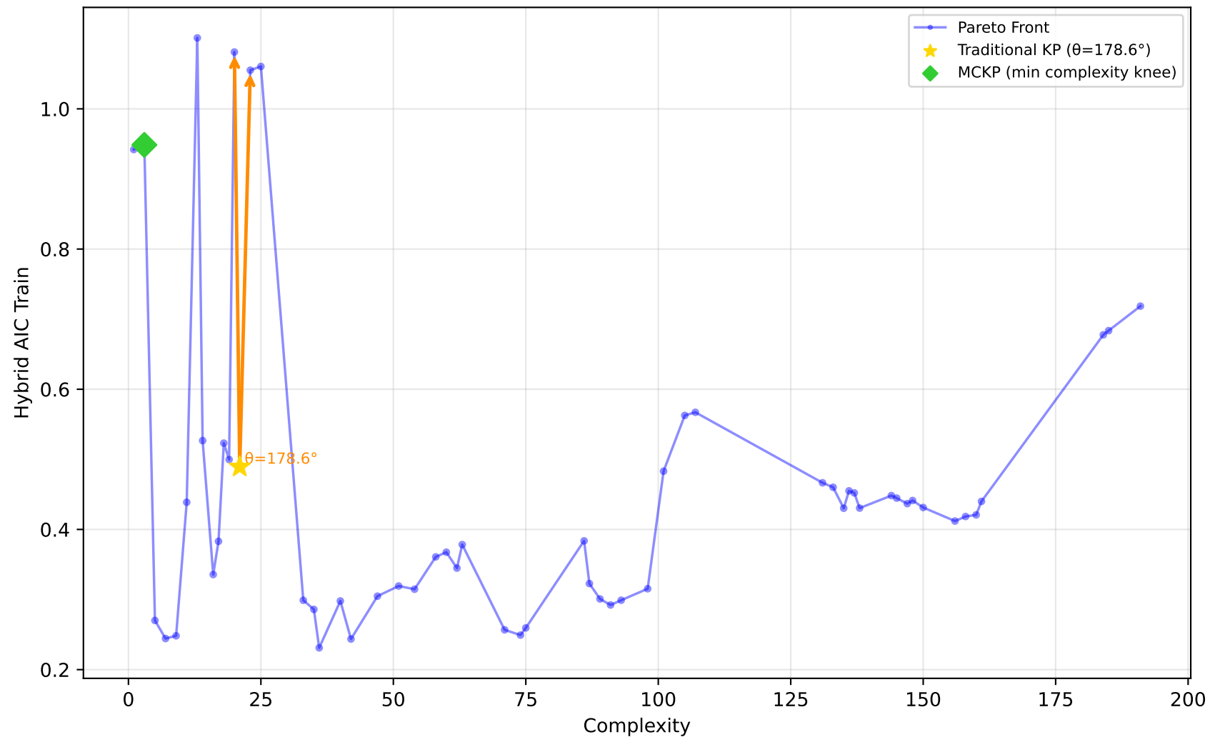
712_chscase_geyser1 - Run 24 - SVP - Hybrid AIC Train \lambda_1=1.00, \lambda_2=1.00, \lambda_3=0.00 | Difficulty: 0.35 | Method: mckp
