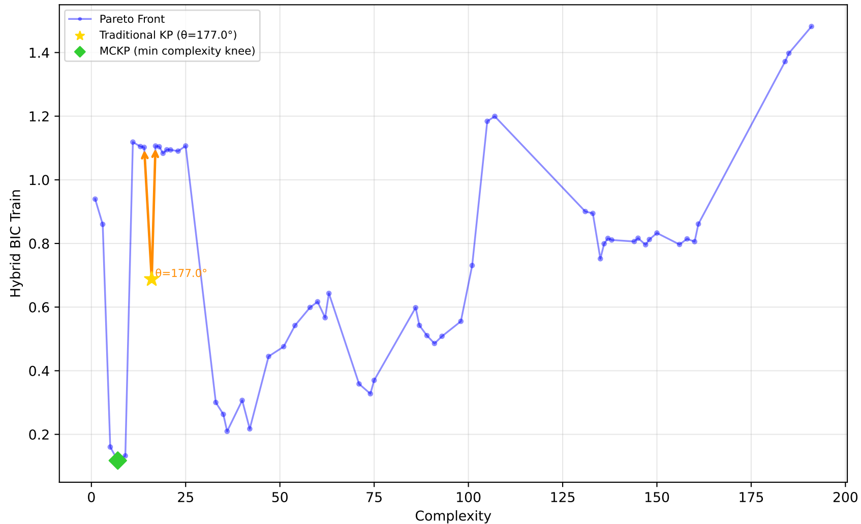
712_chscase_geyser1 - Run 24 - SVP - Hybrid BIC Train \lambda_1=0.00 , \lambda_2=1.00 , \lambda_3=1.00 | Difficulty: 0.35 | Method: mckp
