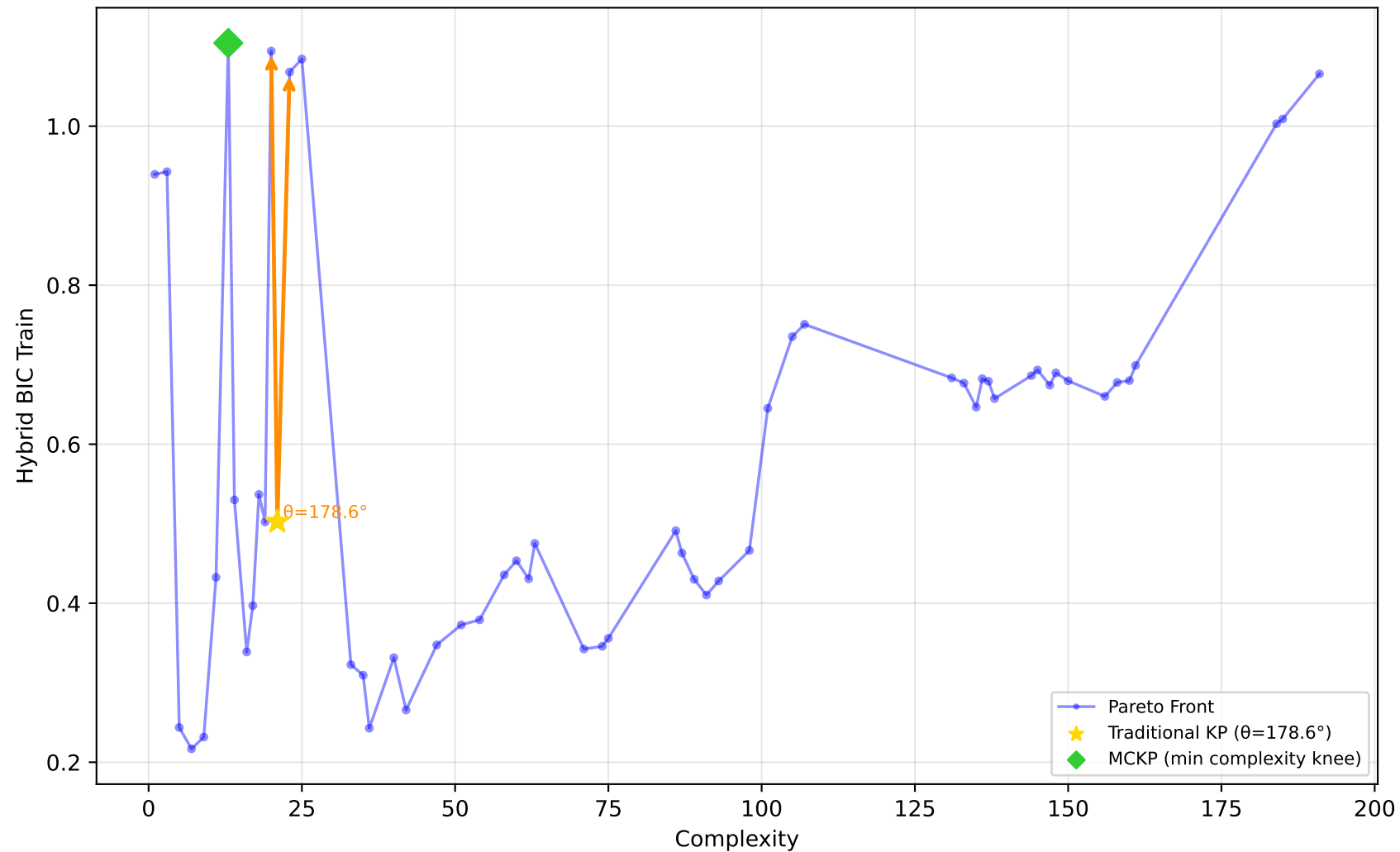
712_chscase_geyser1 - Run 24 - SVP - Hybrid BIC Train \lambda_1=1.00, \lambda_2=1.00, \lambda_3=0.00 | Difficulty: 0.35 | Method: mckp
