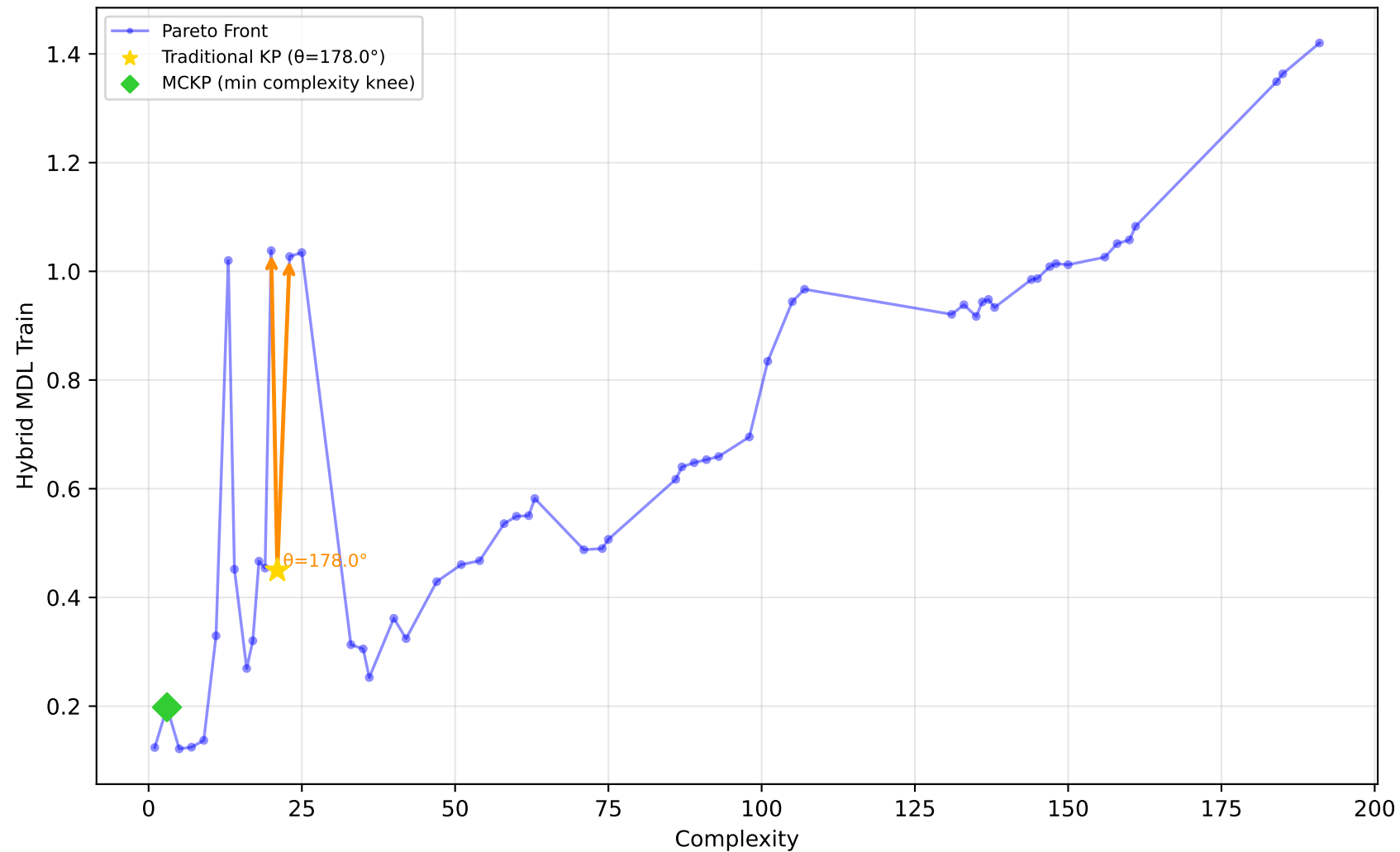
712_chscase_geyser1 - Run 24 - SVP - Hybrid MDL Train \lambda_1=1.00, \lambda_2=1.00, \lambda_3=0.00 | Difficulty: 0.35 | Method: mckp
