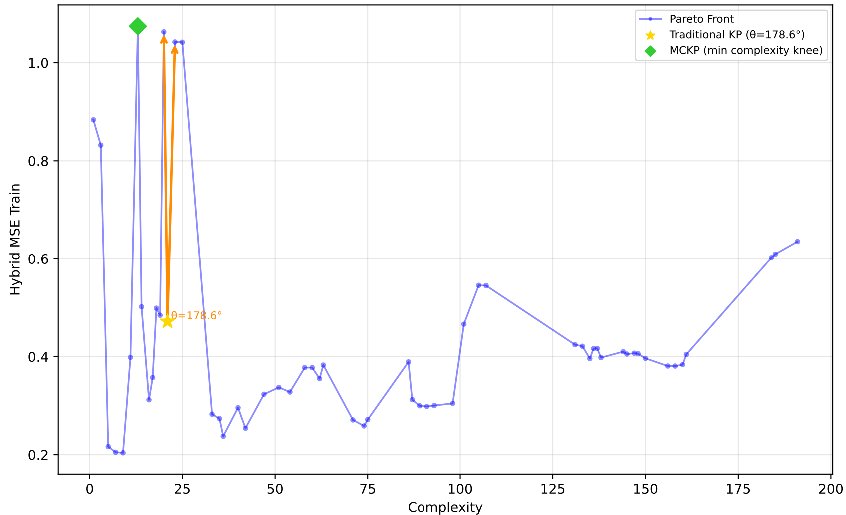
712_chscase_geyser1 - Run 24 - SVP - Hybrid MSE Train \lambda_1=1.00, \lambda_2=1.00, \lambda_3=0.00 | Difficulty: 0.35 | Method: mckp
