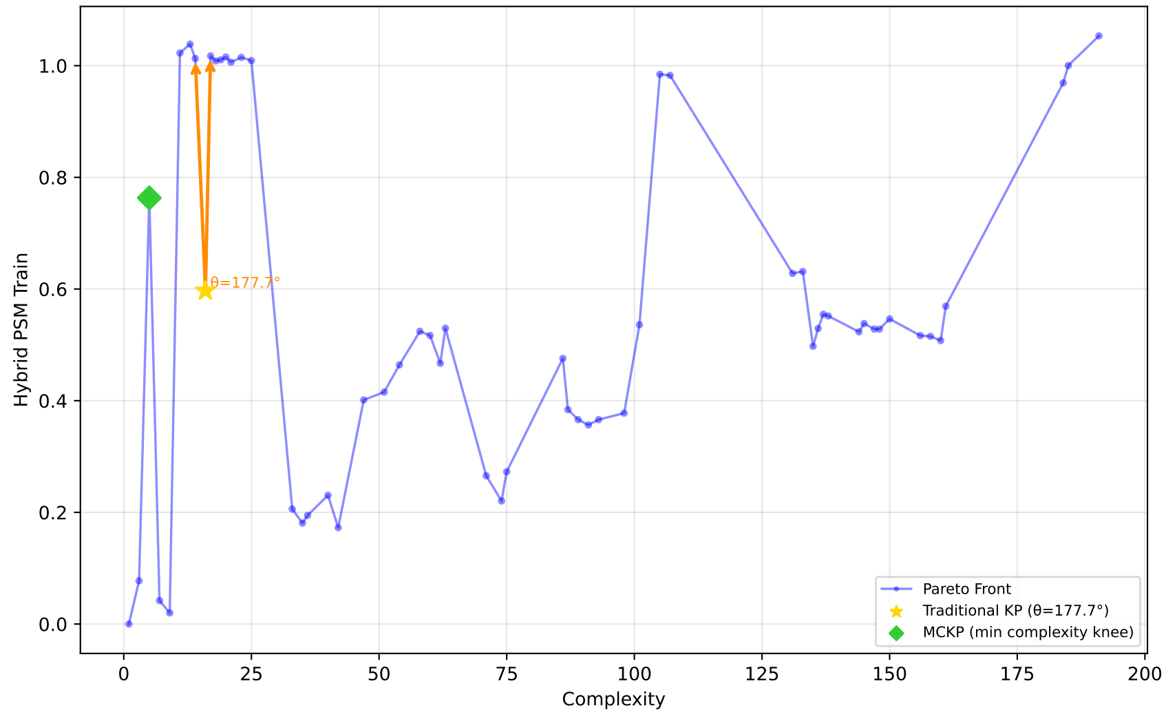
712_chscase_geyser1 - Run 24 - SVP - Hybrid PSM Train \lambda_1=0.00, \lambda_2=1.00, \lambda_3=1.00 | Difficulty: 0.35 | Method: mckp
