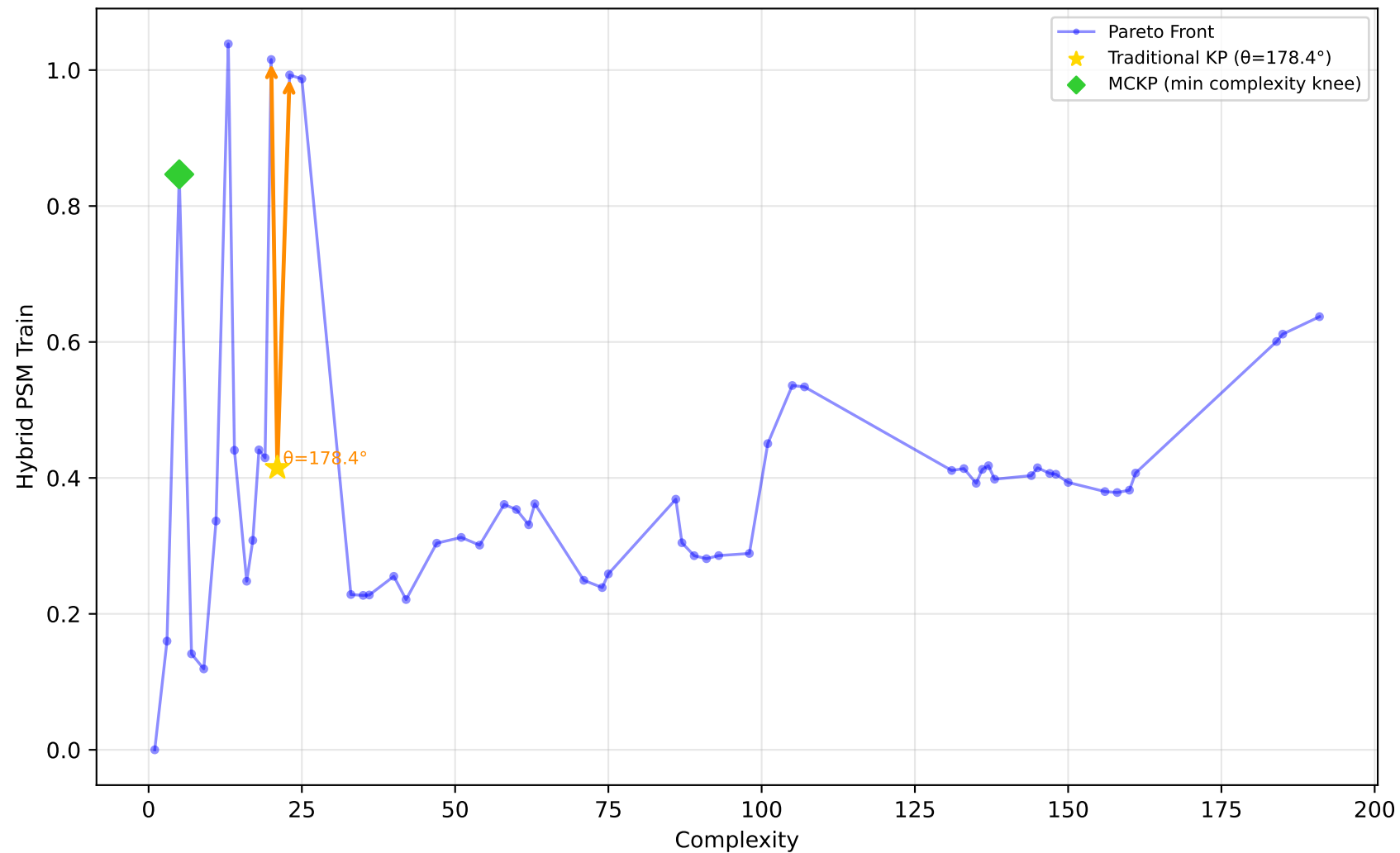
712_chscase_geyser1 - Run 24 - SVP - Hybrid PSM Train \lambda_1=1.00, \lambda_2=1.00, \lambda_3=0.00 | Difficulty: 0.35 | Method: mckp
