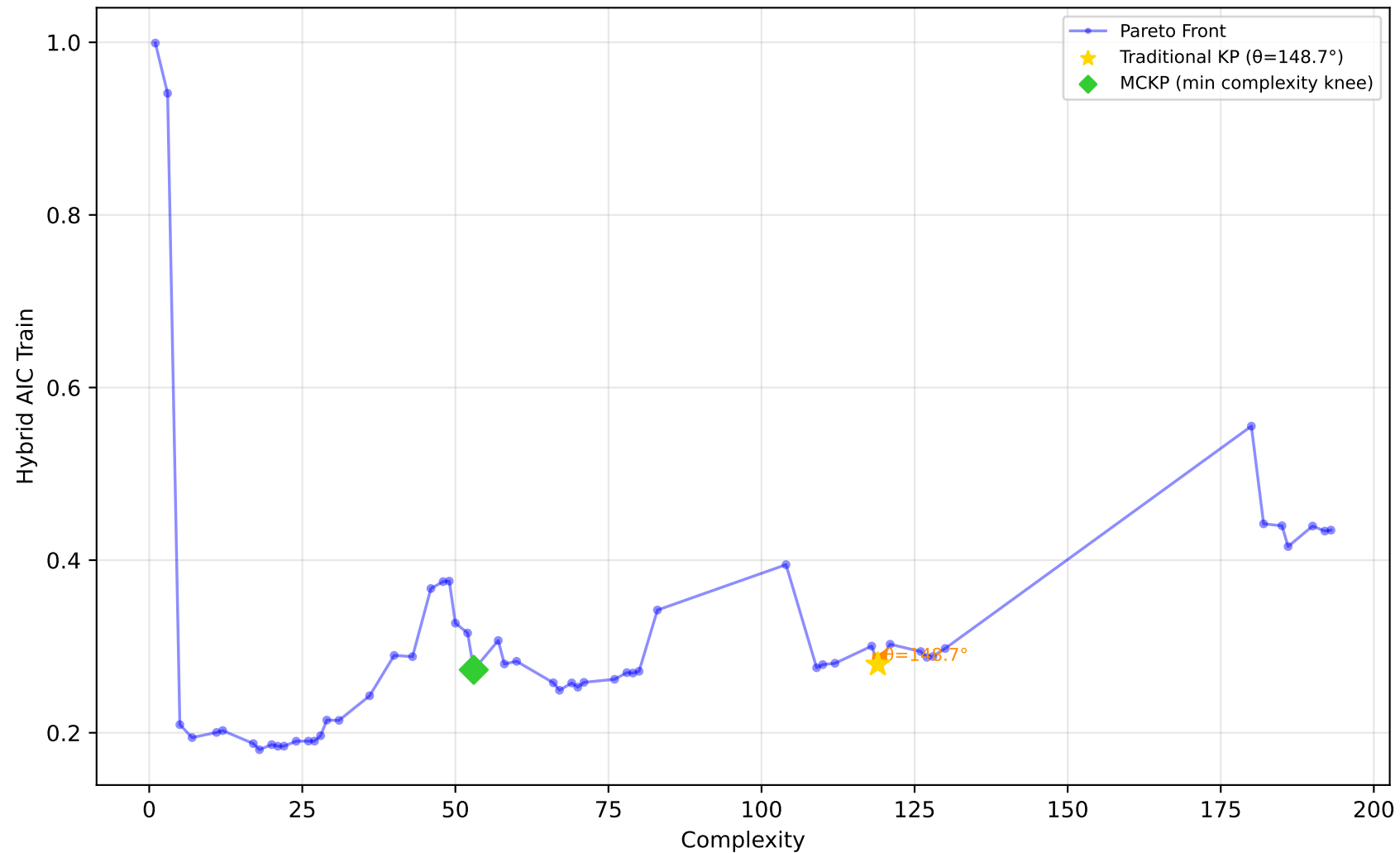
712_chscase_geyser1 - Run 25 - MVP - Hybrid AIC Train \lambda_1=0.20, \lambda_2=1.00, \lambda_3=1.00 | Difficulty: 0.84 | Method: hmr
