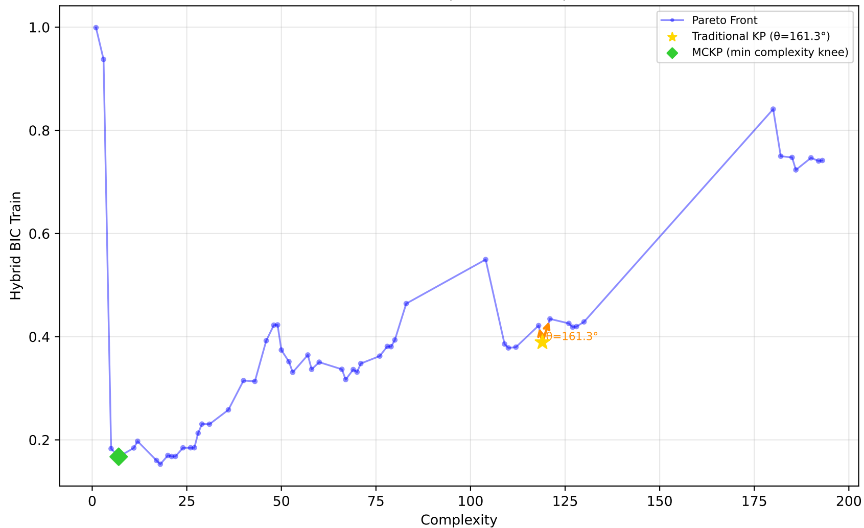
712_chscase_geyser1 - Run 25 - MVP - Hybrid BIC Train \lambda_1=0.20, \lambda_2=1.00, \lambda_3=1.00 | Difficulty: 0.84 | Method: hmr
