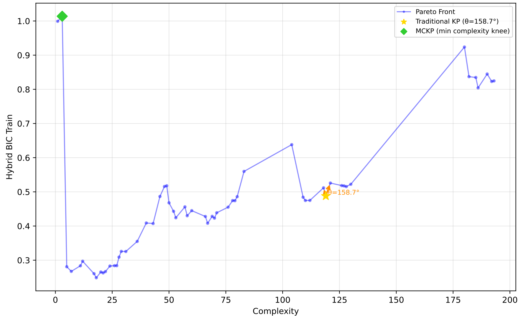
712_chscase_geyser1 - Run 25 - MVP - Hybrid BIC Train \lambda_1=1.00, \lambda_2=1.00, \lambda_3=1.00 | Difficulty: 0.84 | Method: hmr
