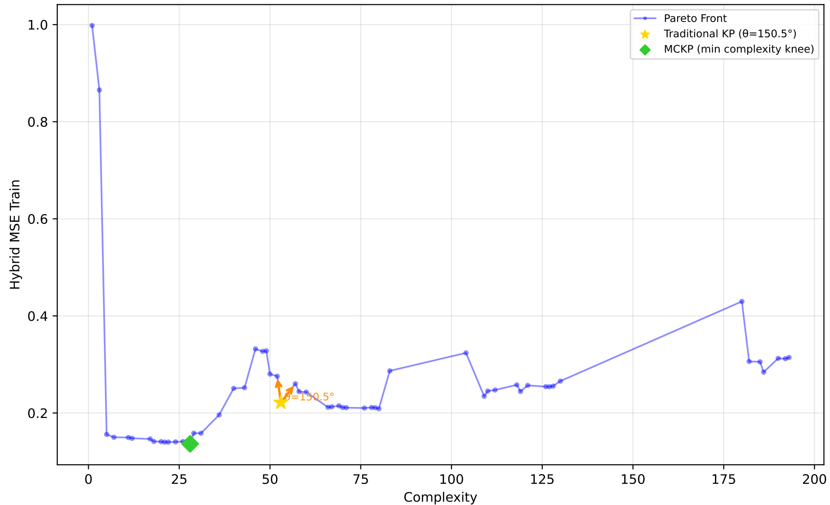
712_chscase_geyser1 - Run 25 - MVP - Hybrid MSE Train \lambda_1=0.20, \lambda_2=1.00, \lambda_3=1.00 | Difficulty: 0.84 | Method: hmr
