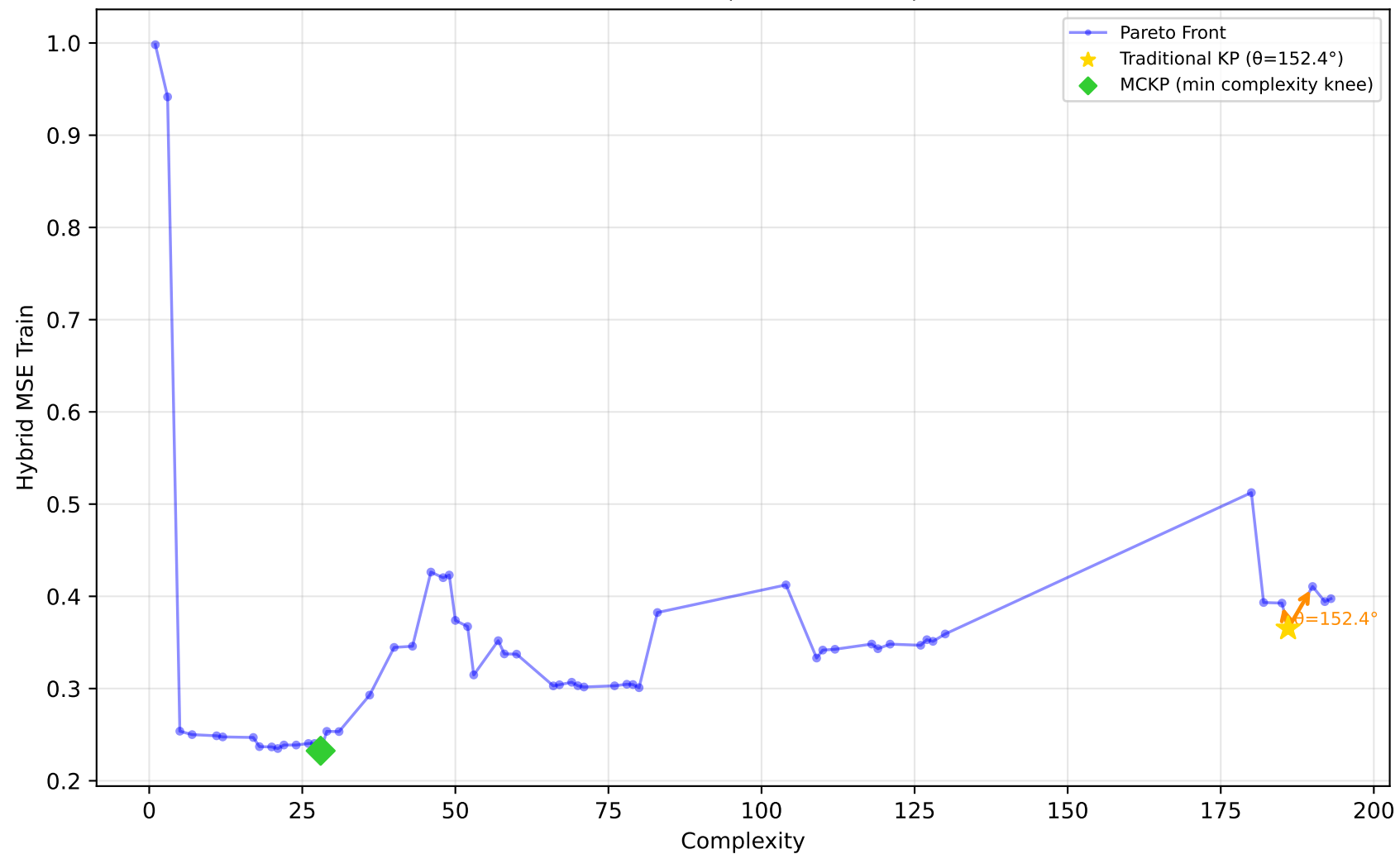
712_chscase_geyser1 - Run 25 - MVP - Hybrid MSE Train \lambda_1=1.00, \lambda_2=1.00, \lambda_3=1.00 | Difficulty: 0.84 | Method: hmr
