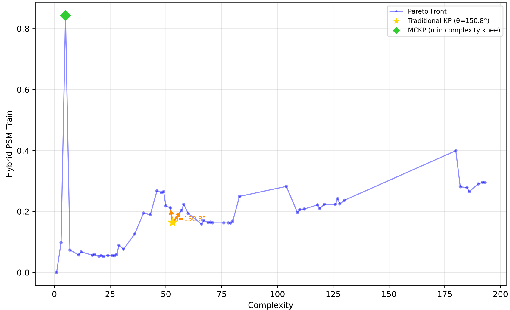
712_chscase_geyser1 - Run 25 - MVP - Hybrid PSM Train \lambda_1=0.20, \lambda_2=1.00, \lambda_3=1.00 | Difficulty: 0.84 | Method: hmr
